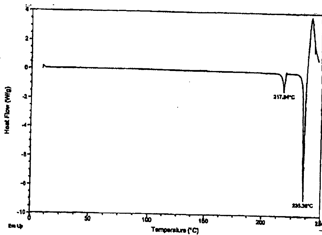
Fig. 5a: Differential Scanning Calorimetry (DSC) of the anhydrous Form B of Example 2
