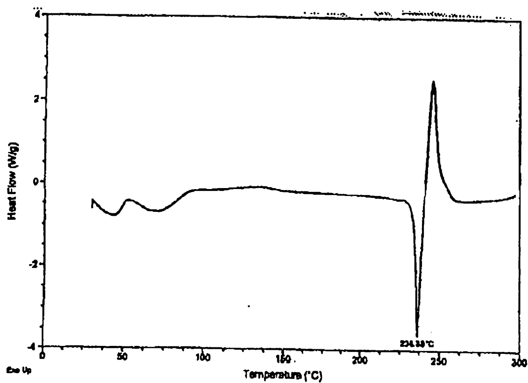
Fig. 6a: Differential Scanning Calorimetry (DSC) of the dihydrate form C of Example 2
