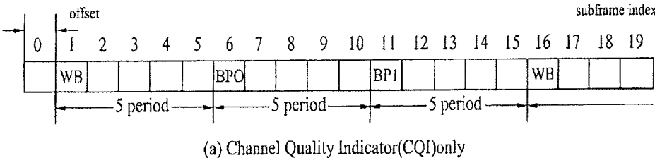
(a) Channel Quality Indicator(CQI)only
