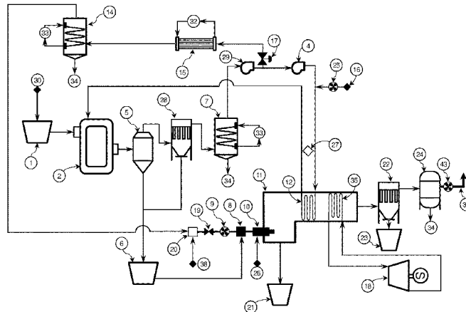
Block Diagram of Treatment System 100
