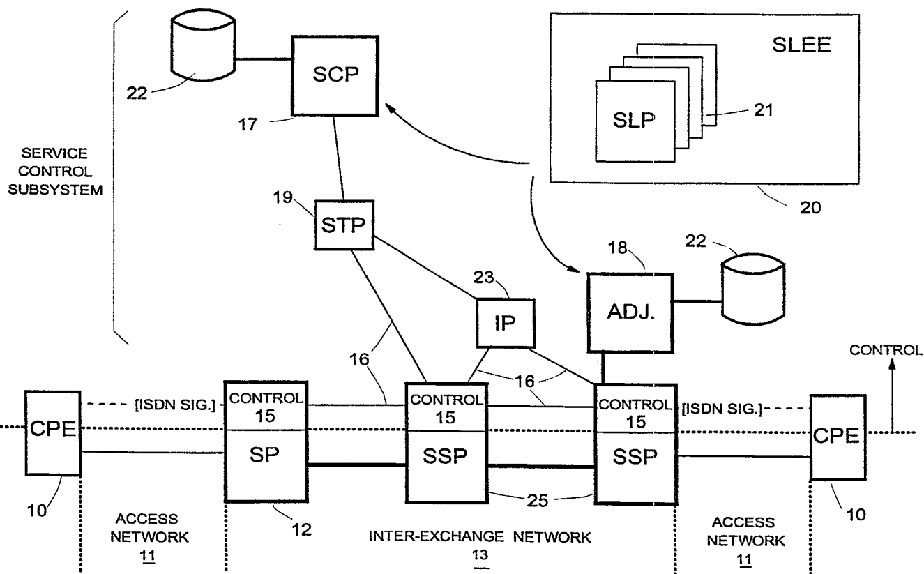
FIG. 2 (PRIOR ART)
