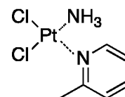
Picoplatin
