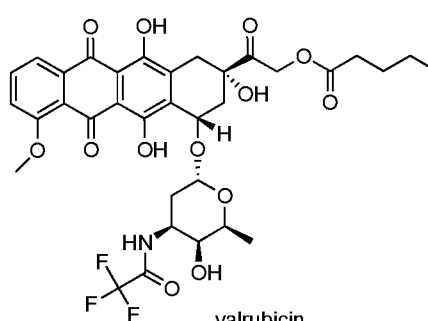
valrubicin
