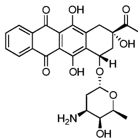
idarubicin
