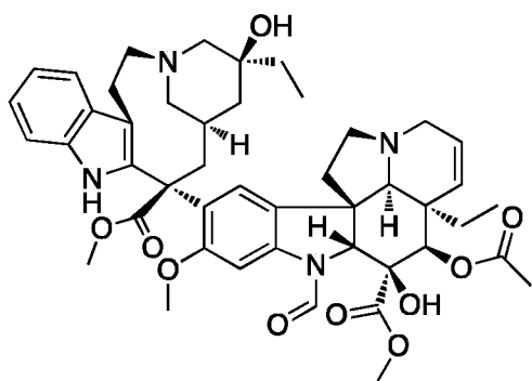
Vincristine
