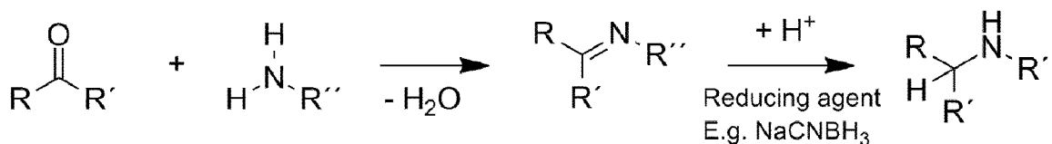
Scheme 4. Reductive amination
