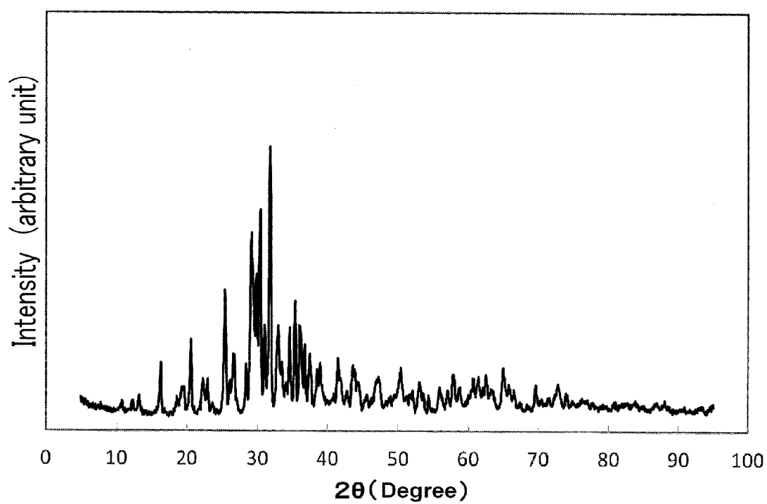
Powder XRD pattern of example 8 (Actually measured)
