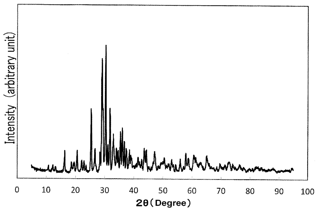
Powder XRD pattern of example 9 (Actually measured)
