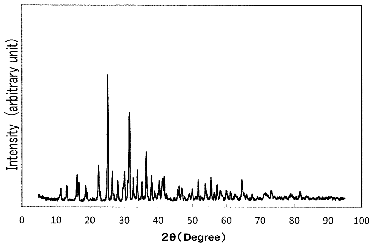
Powder XRD pattern of example 32 (Actually measured)
