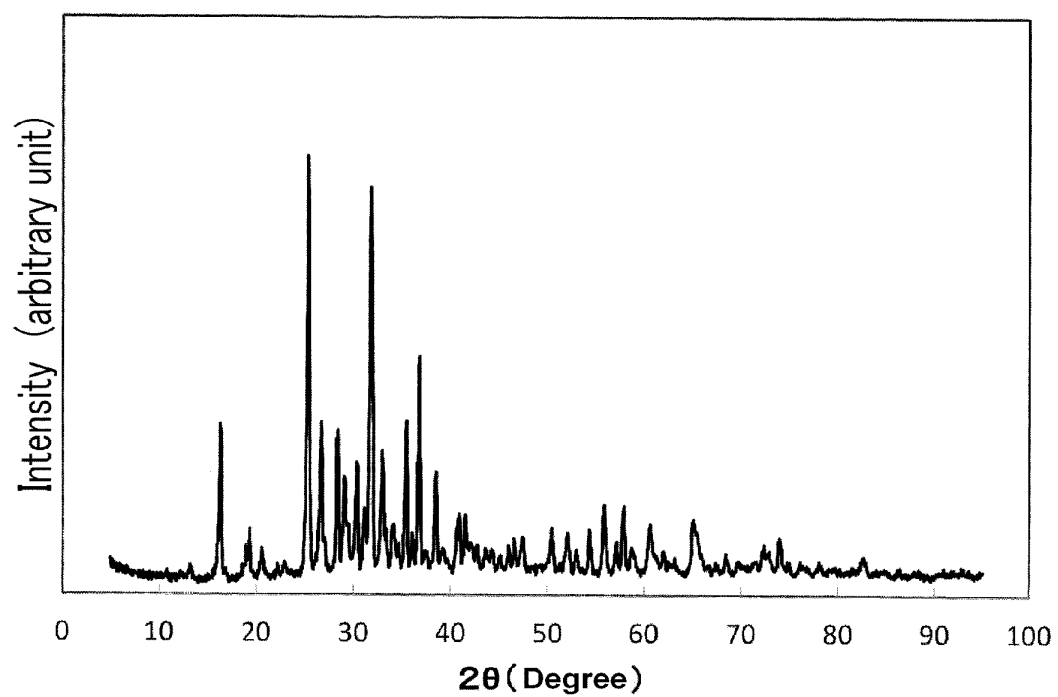
Powder XRD pattern of example 2 (Actually measured)
