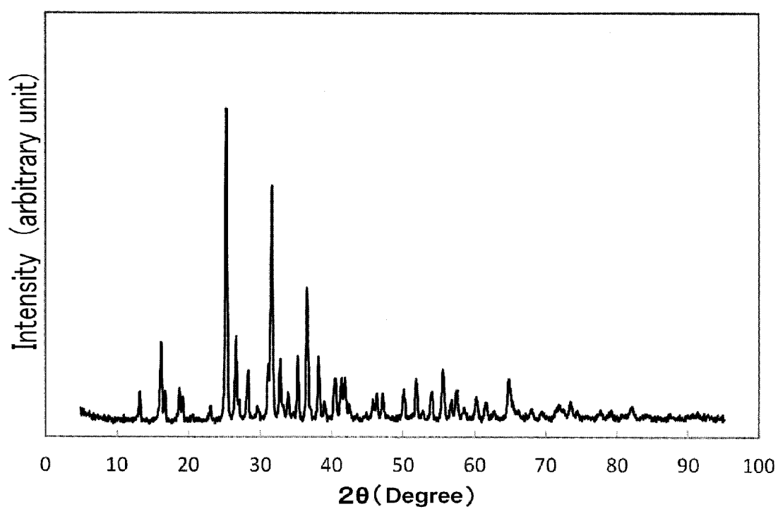
Powder XRD pattern of example 57 (Actually measured)
