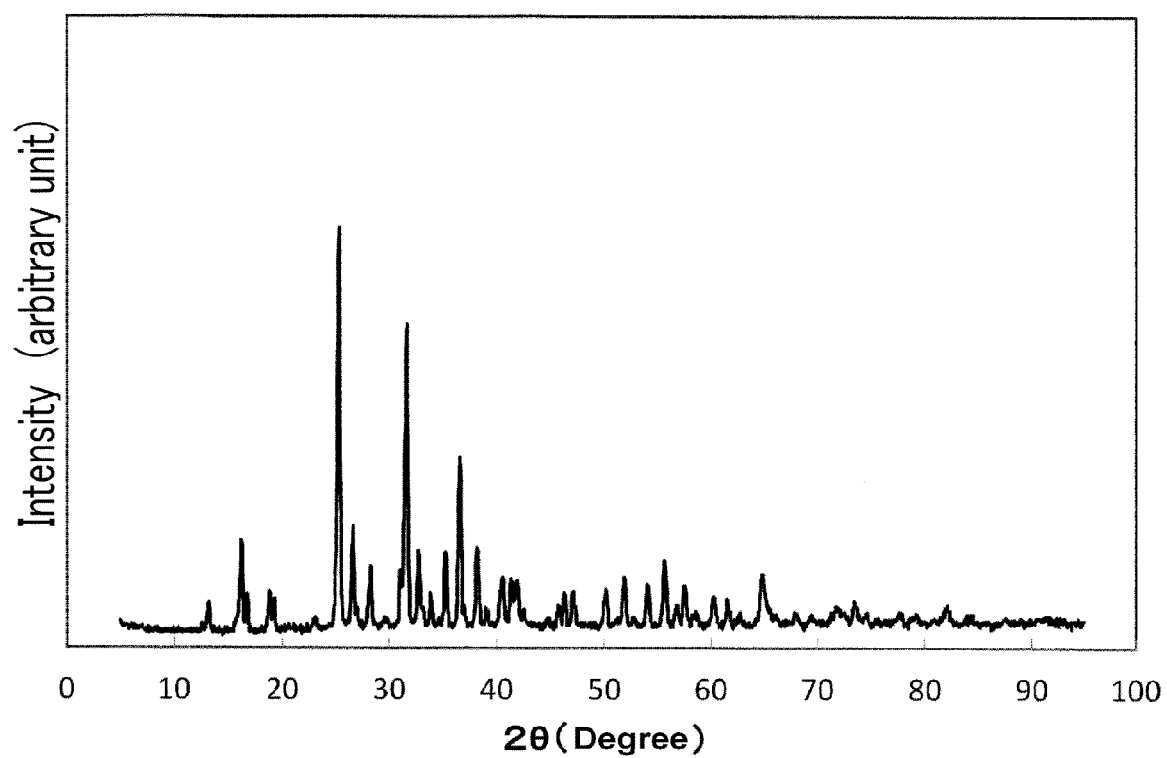
Powder XRD pattern of example 41 (Actually measured)
