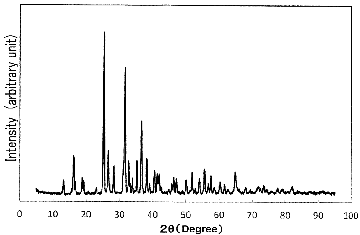
Powder XRD pattern of example 7 (Actually measured)
