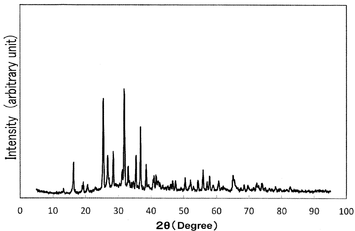
Powder XRD pattern of example 26 (Actually measured)
