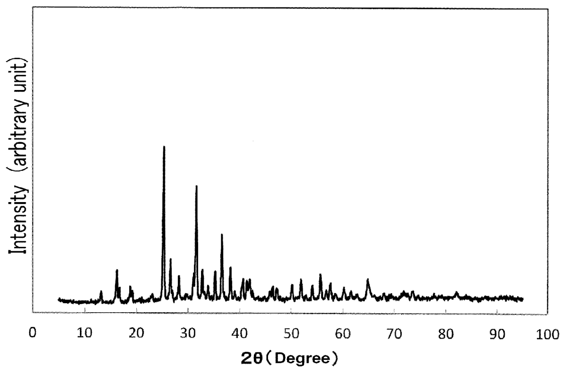
Powder XRD pattern of example 25 (Actually measured)
