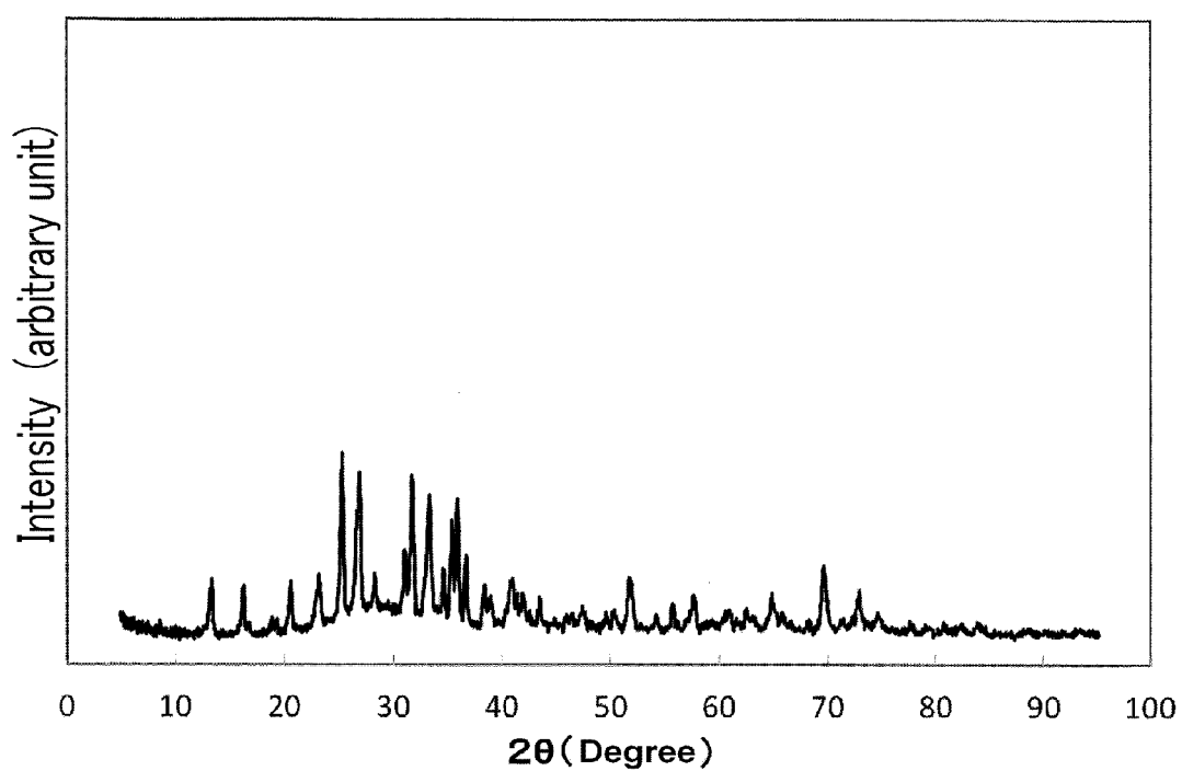
Powder XRD pattern of example 36 (Actually measured)
