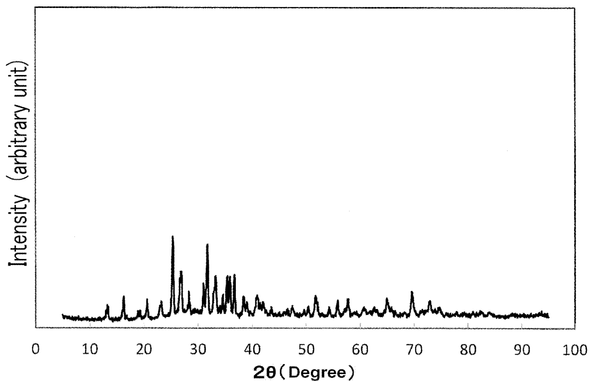
Powder XRD pattern of example 56 (Actually measured)
