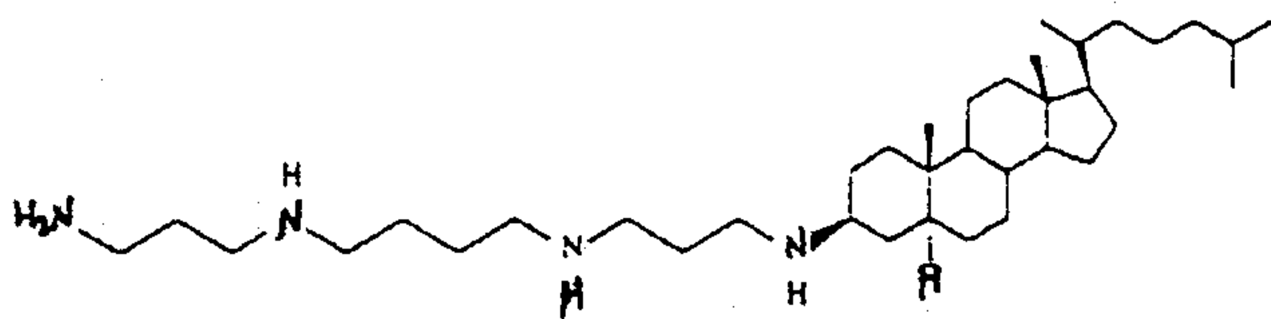
Compound 353
