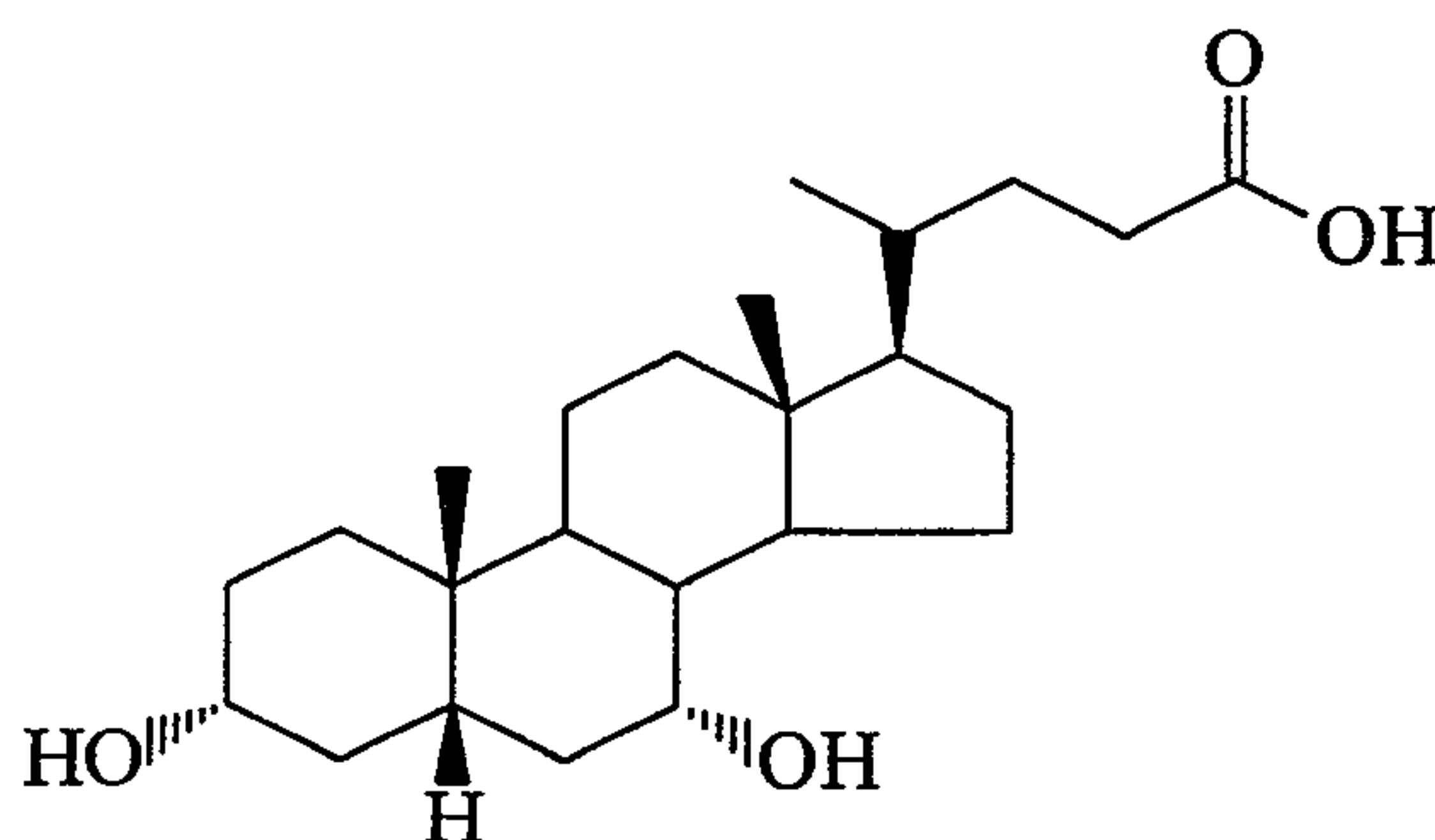
Chenodeoxycholic Acid
