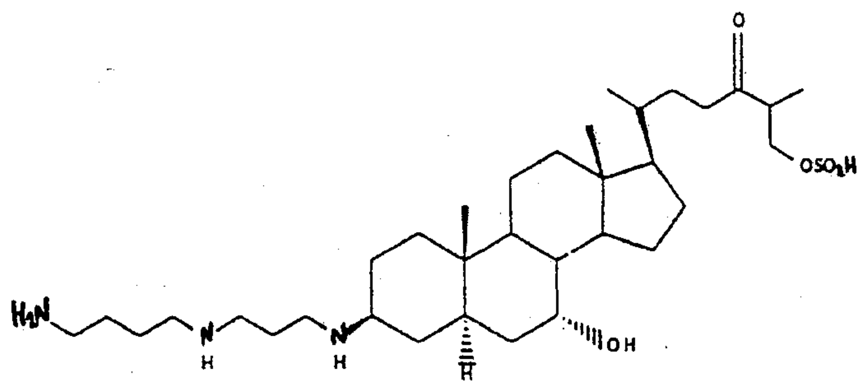
Compound 1360
