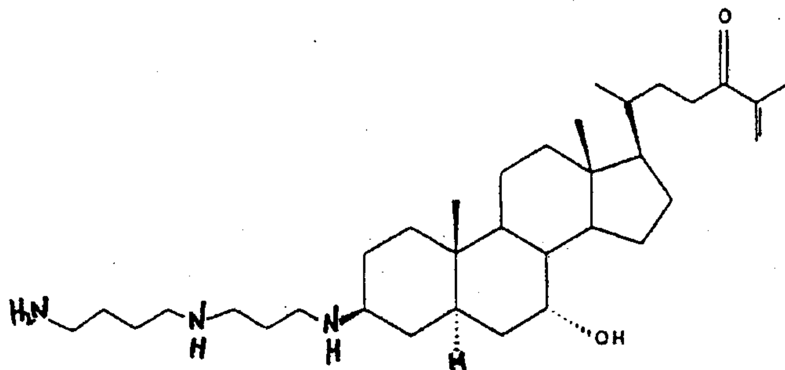
Compound 1361
