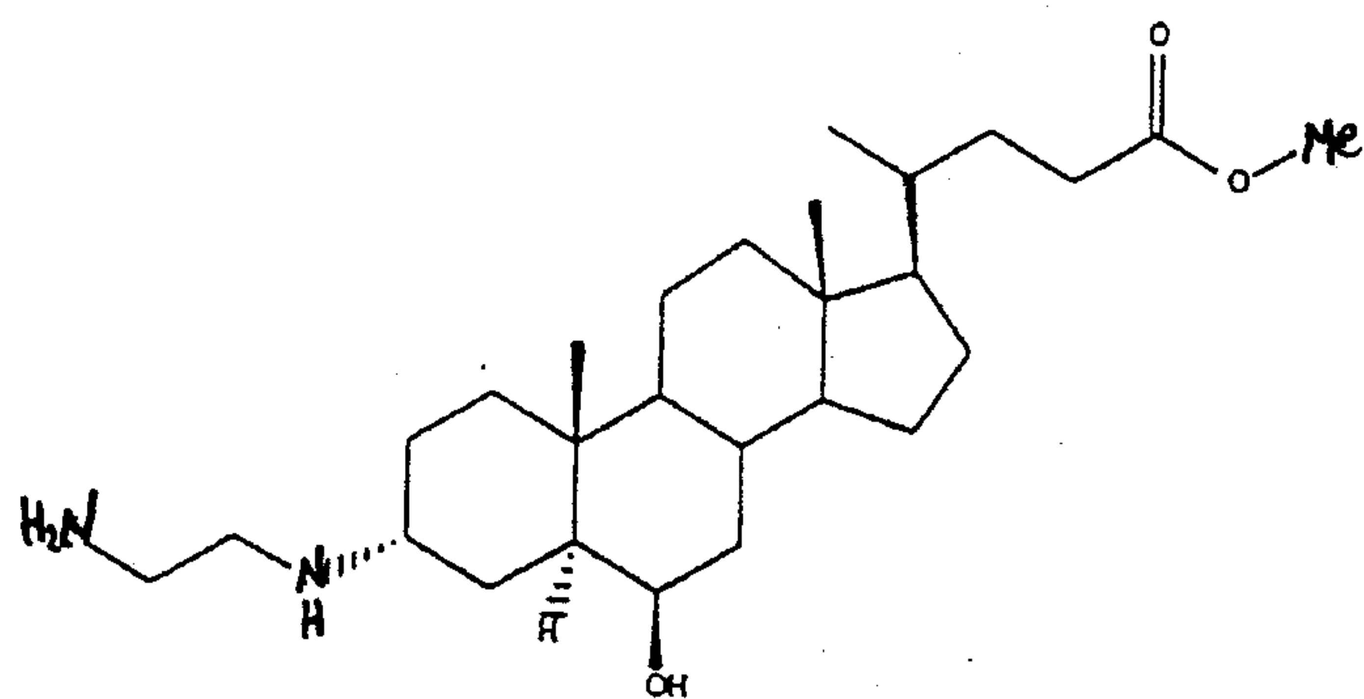
Compound 431
