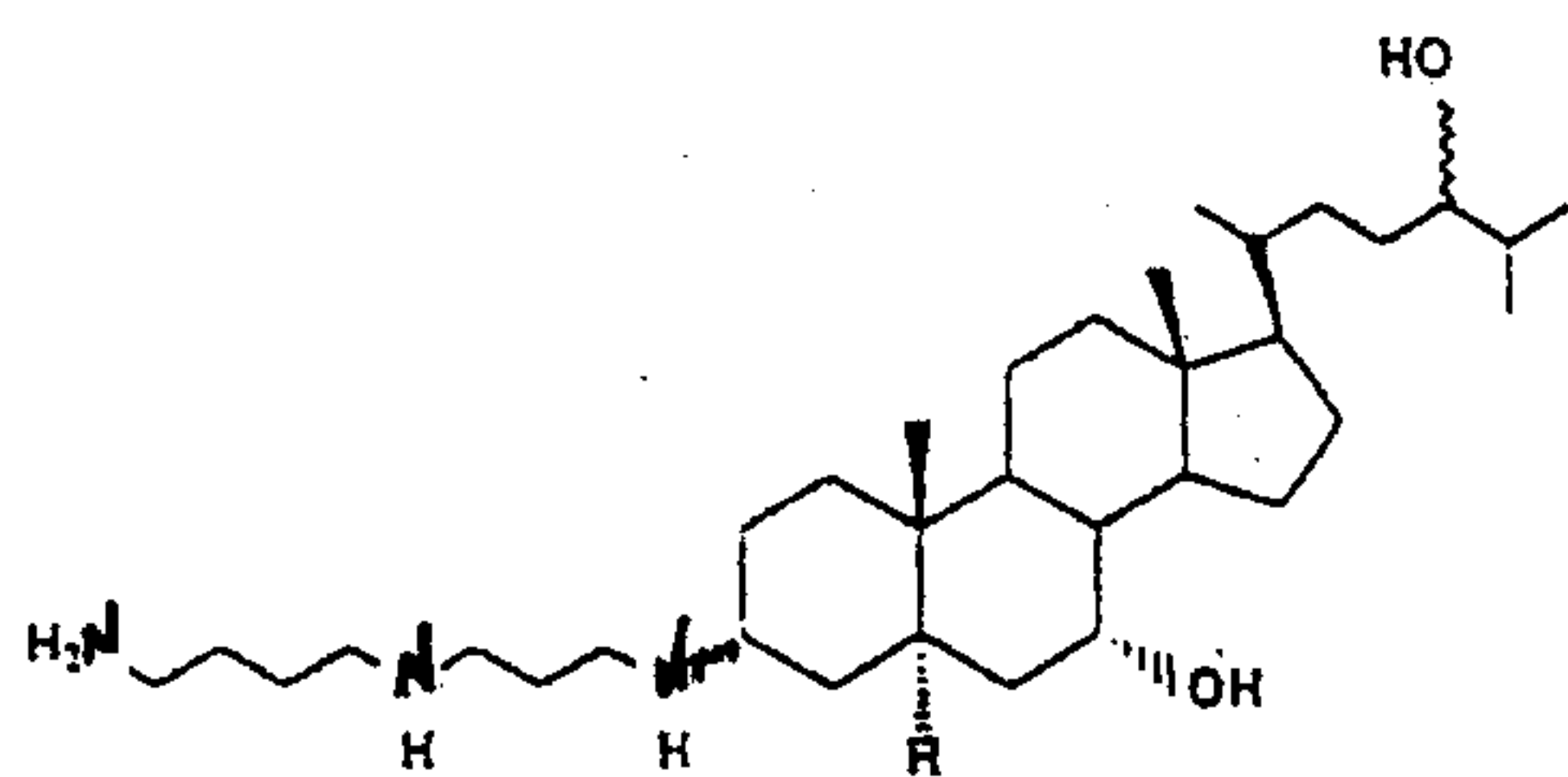
Compound 387
