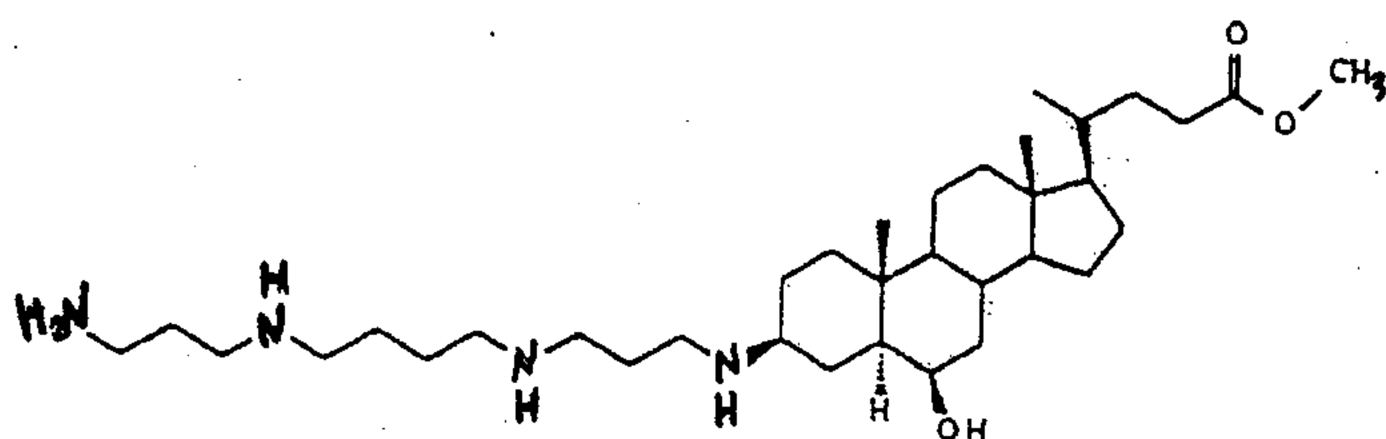
Compound 466
