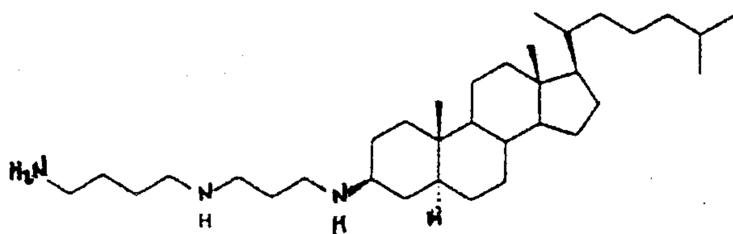
Compound 303
