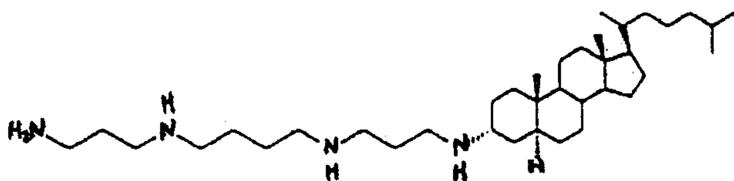
Compound 354
