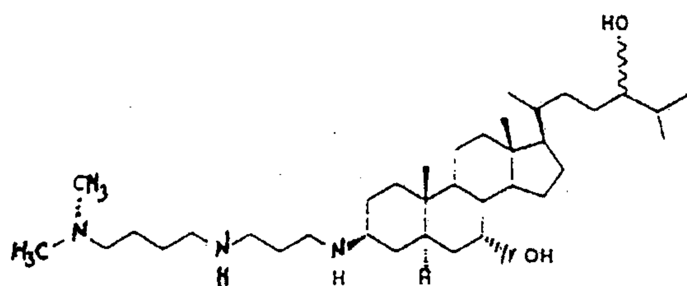
MSI- 1239A
