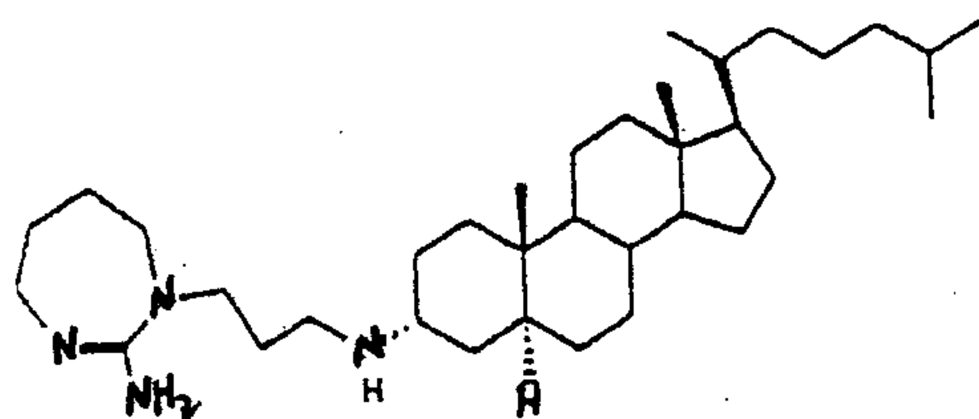
Compound 393
