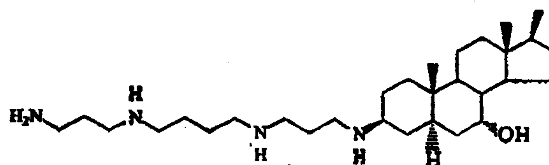
STERIOD B
