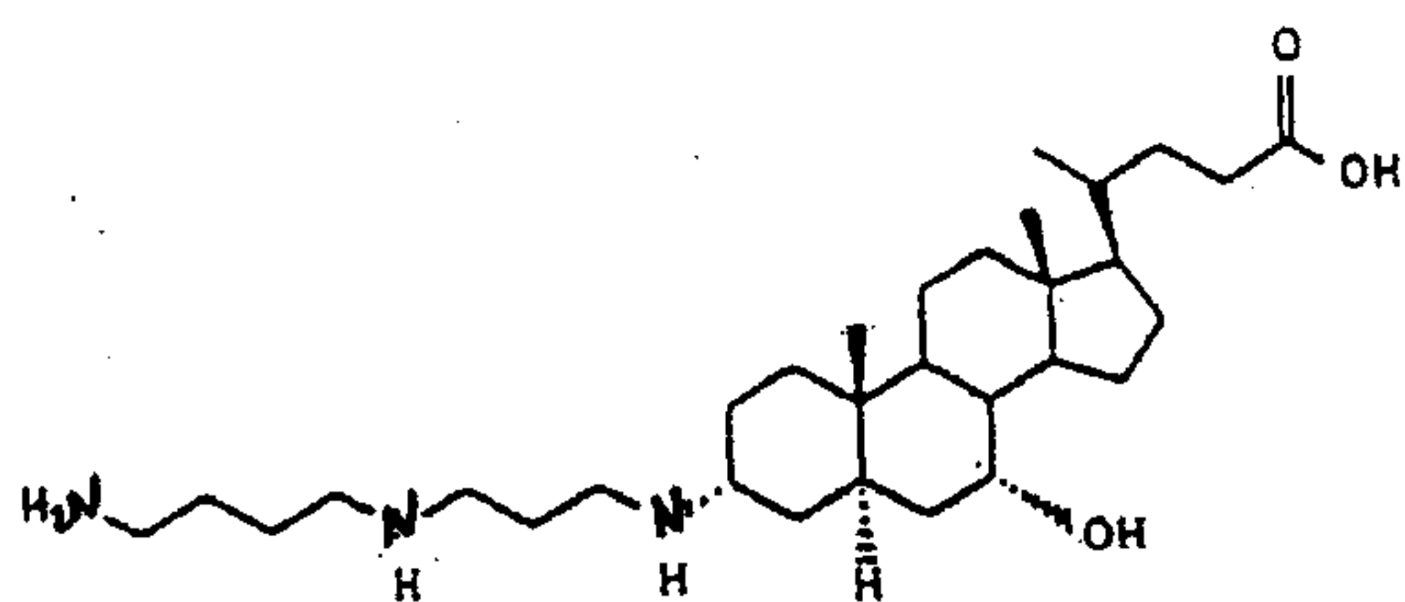
Compound 382
