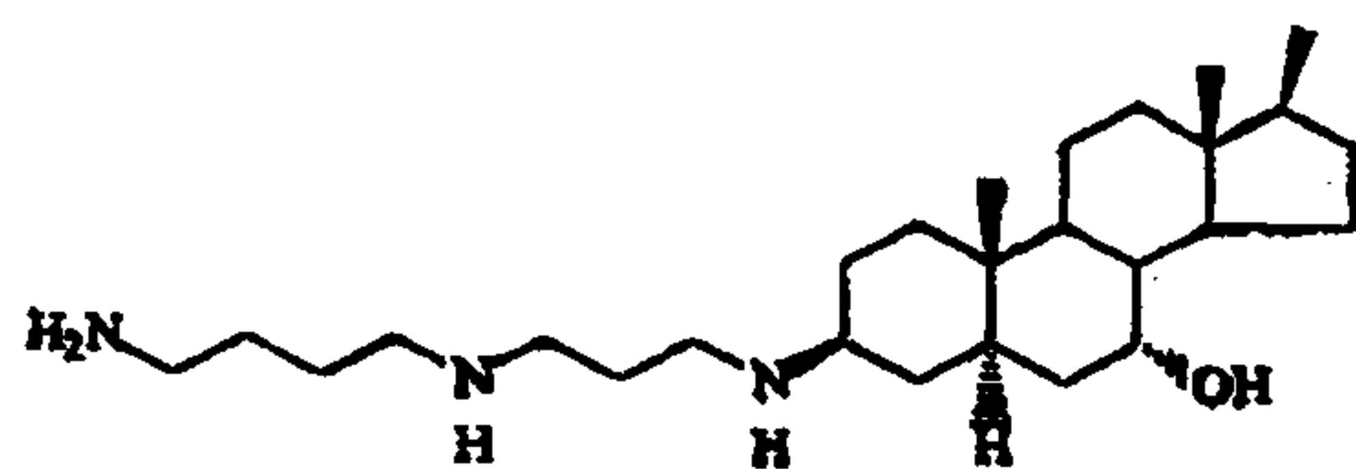
STEROID A
