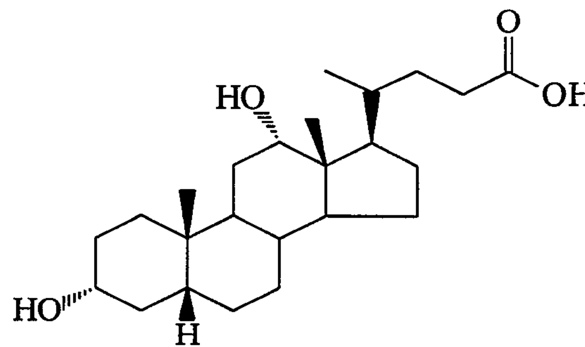
Deoxycholic Acid
