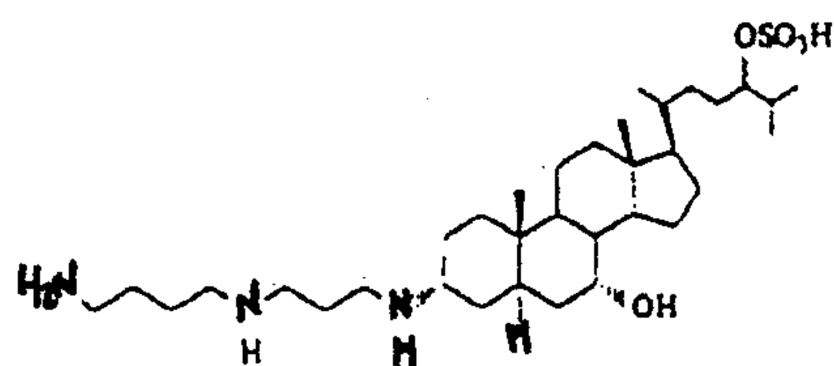
Compound 388
