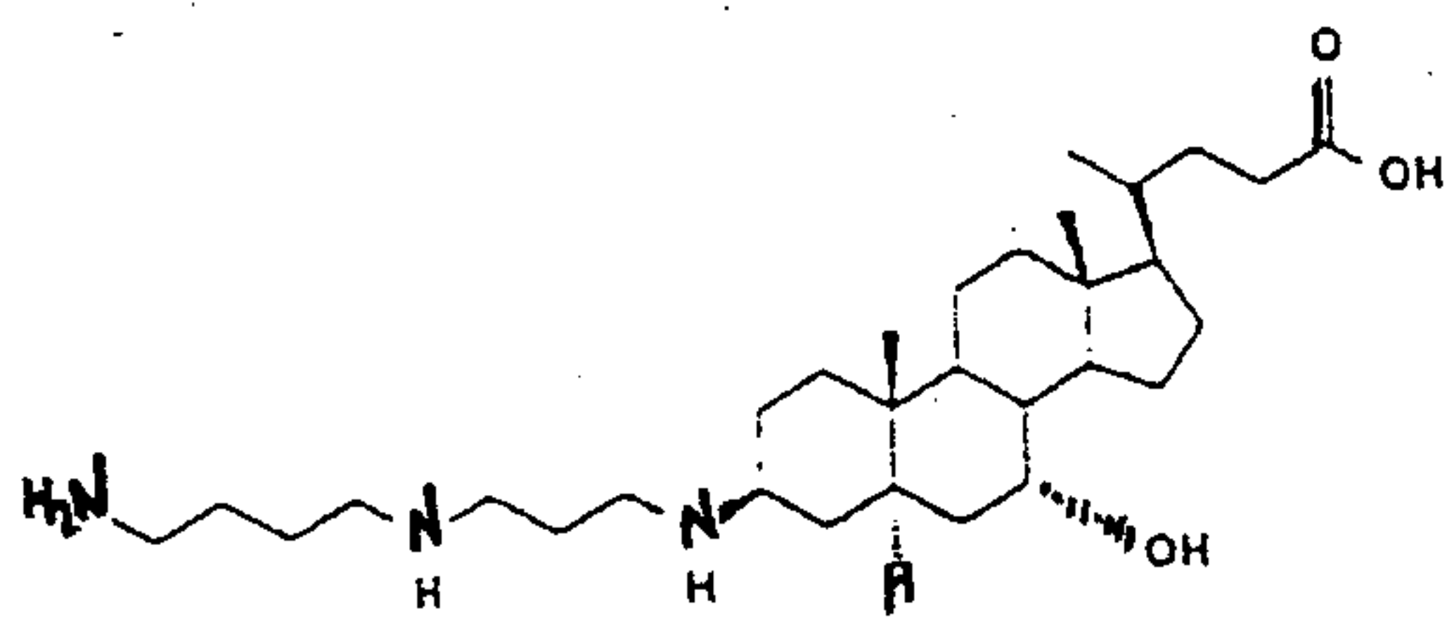
Compound 381
