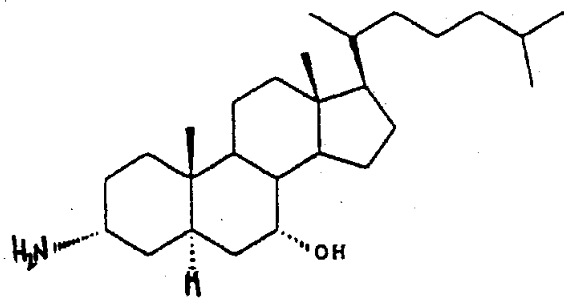
Compound 1363
