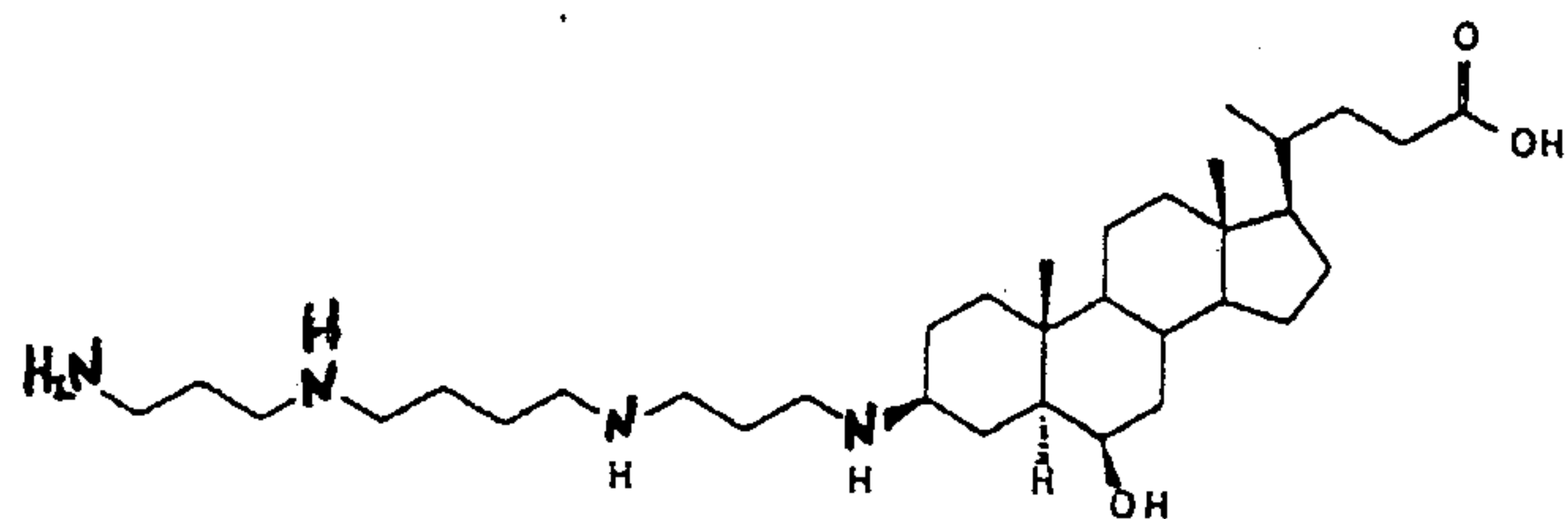
Compound 467
