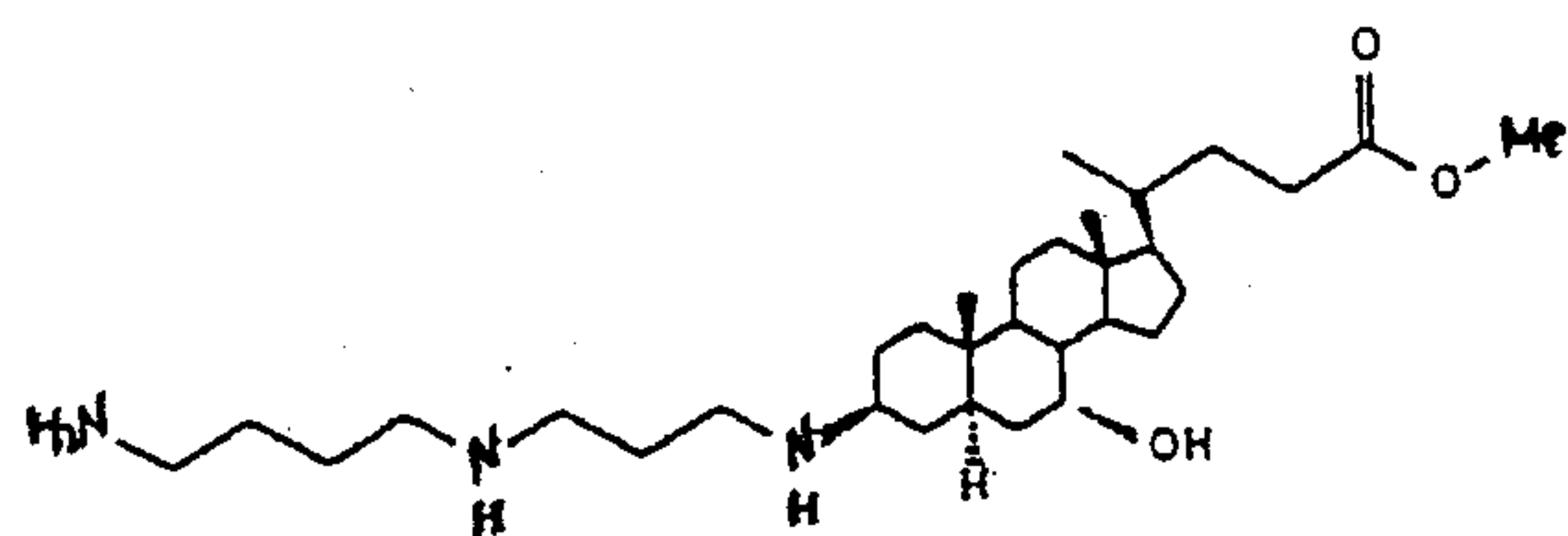
Compound 380
