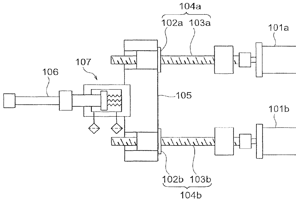
FIG. 6 PRIOR ART
