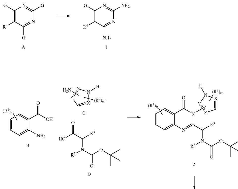
Reaction Scheme 1
