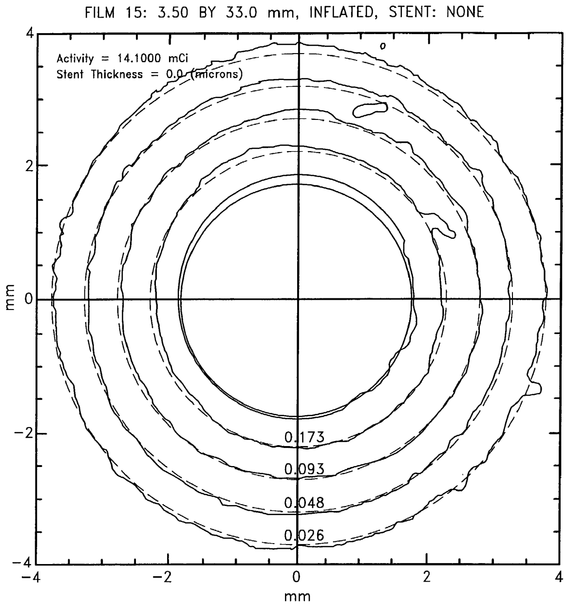
GafCHRONIC FILM DOSE CONTOURS [GRAY/mCi-min]
