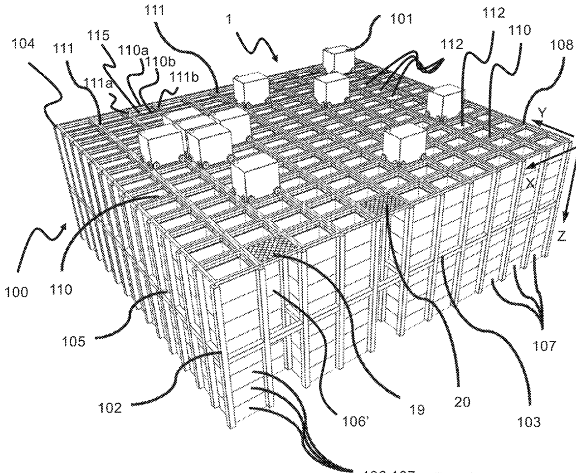
106,107 Fig. 1 (Prior Art)
