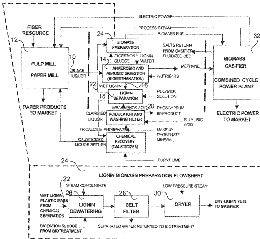
SCHMATIC DESCRIPTION OF LIGNIN PREPARATION PROCESS
