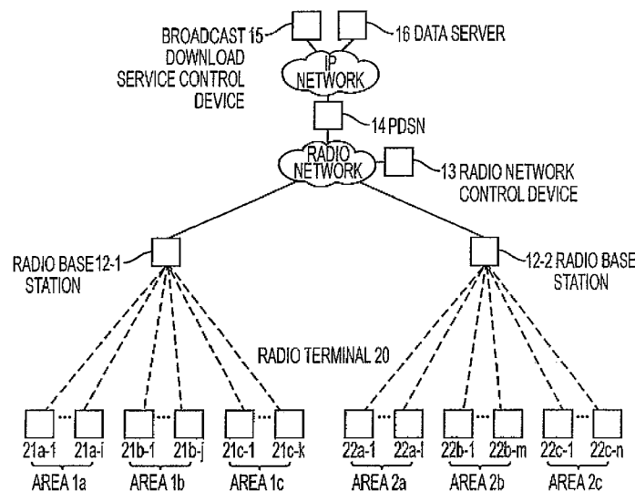
EXAMPLE OF INFORMATION TRANSMITTING SYSTEM
