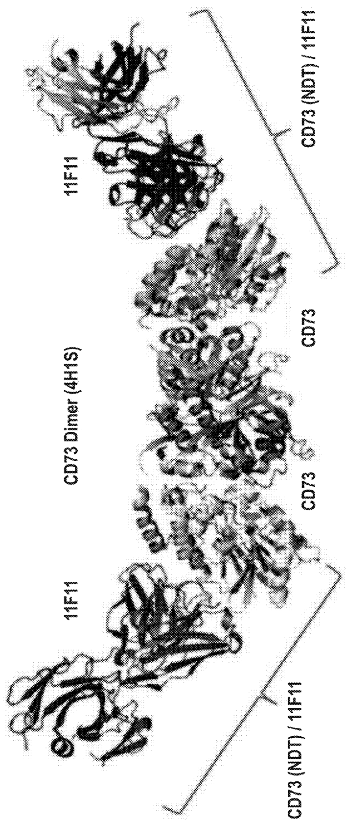
Composite structure of two CD73(NDT)/11F11 complexes superimposed on CD73 dimer (PDP Entry 4H1S)
