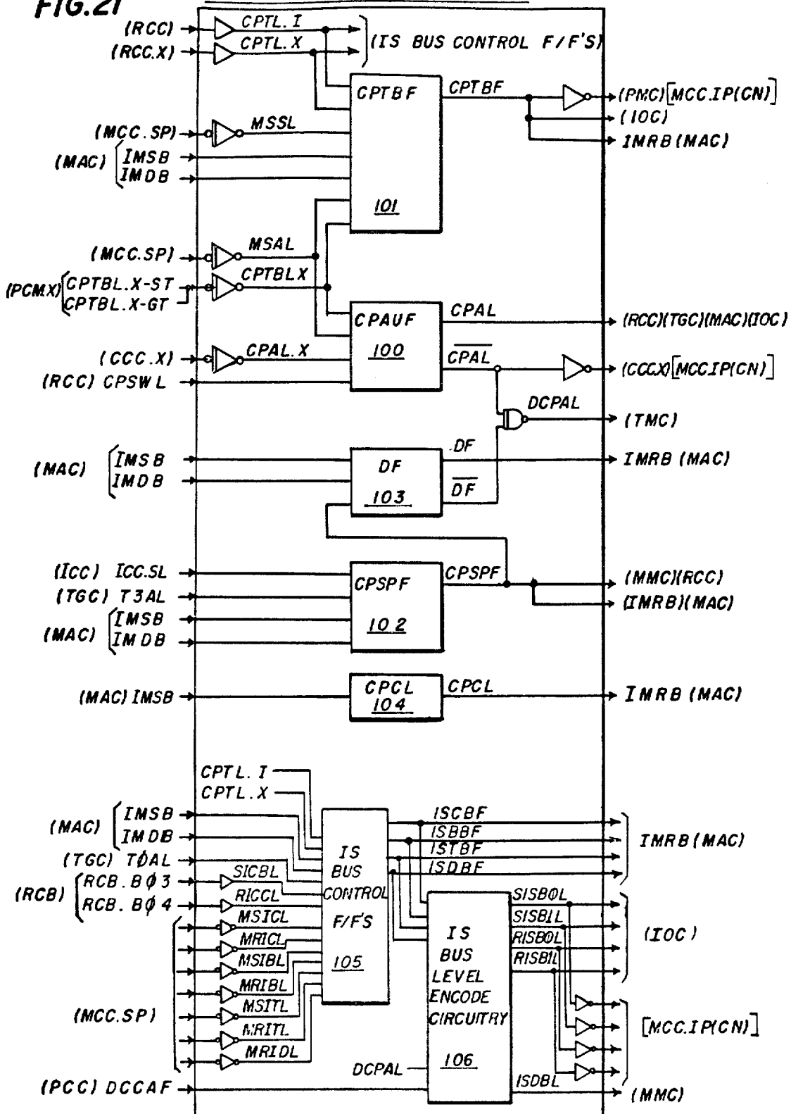
CCC FUNCTIONAL BLOCK DIAGRAM
