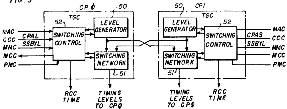
TIMING GENERATOR CIRCUIT
