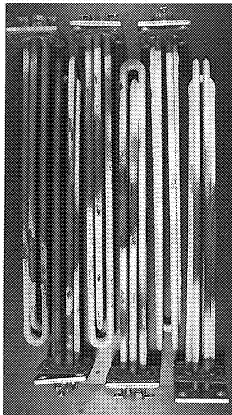
Booster heater with treated water
