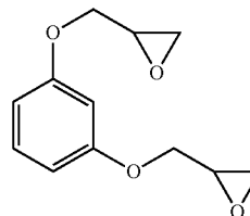
Resorcinol diglycidyl ether
