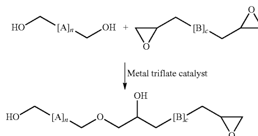
Reaction scheme 1
