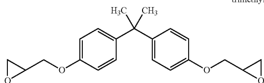
Bisphenol A diglycidyl ether
