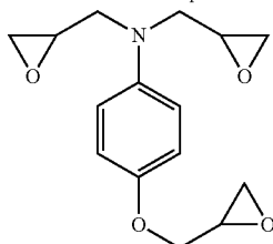
N,N-Diglycidyl-4-glycidyoxyaniline
