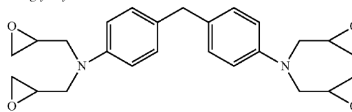
4,4'-Methylenebis(N,N-diglycidylaniline)
