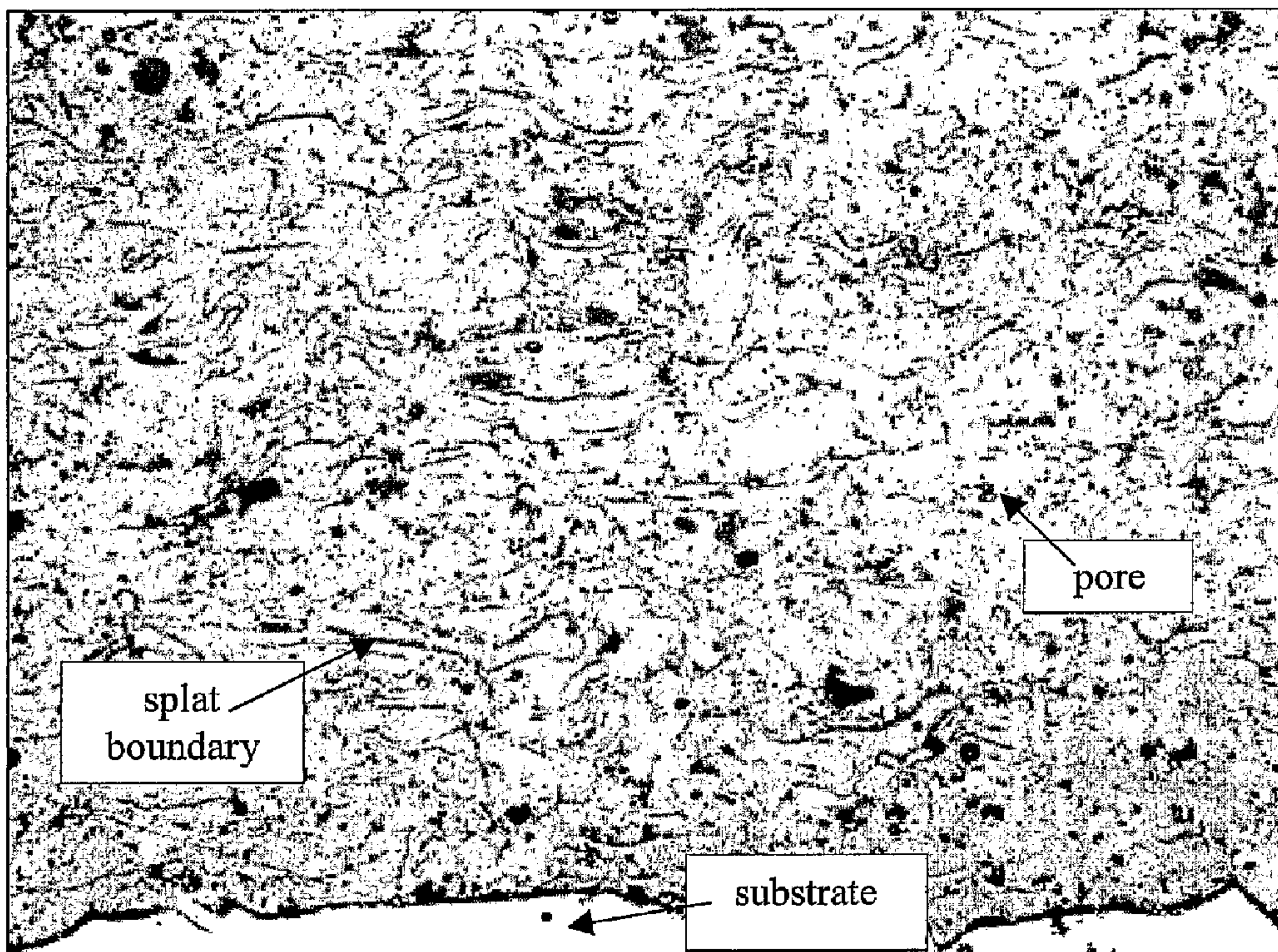
Pre-alloyed YSZ coating A 11.8% Porosity 200x
