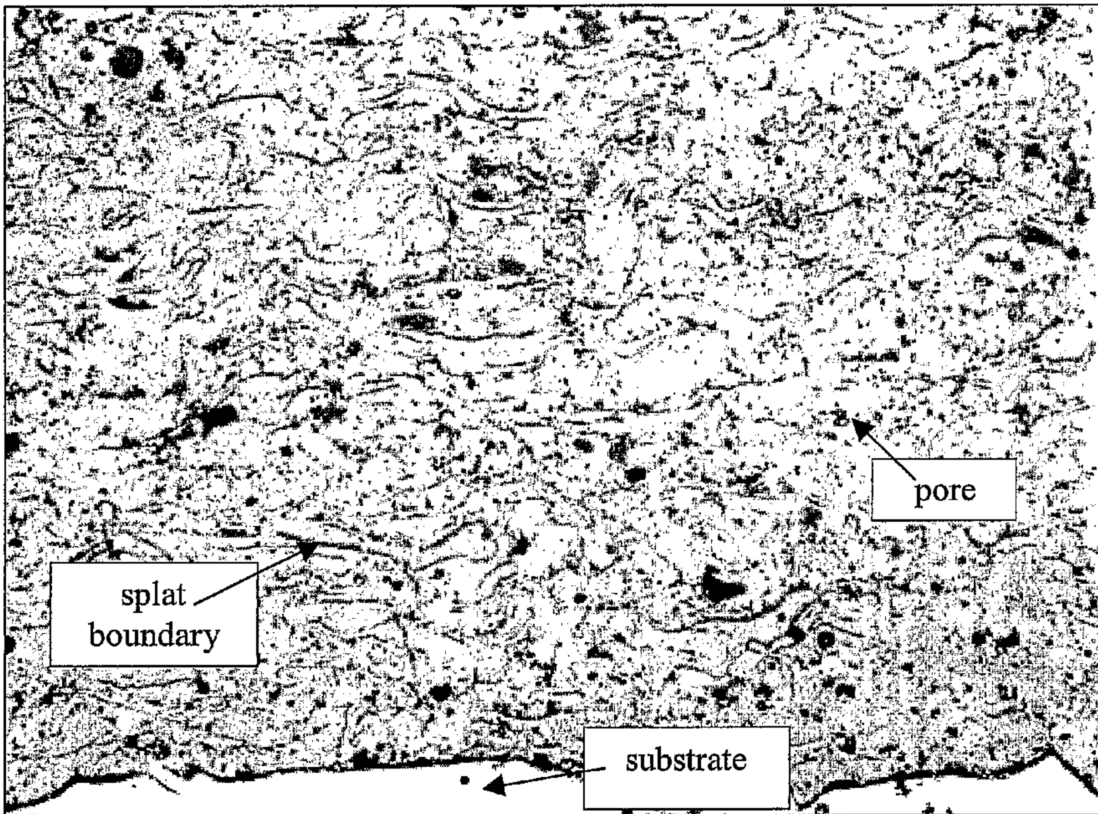
Pre-alloyed YSZ coating A 11.8% Porosity 200x
