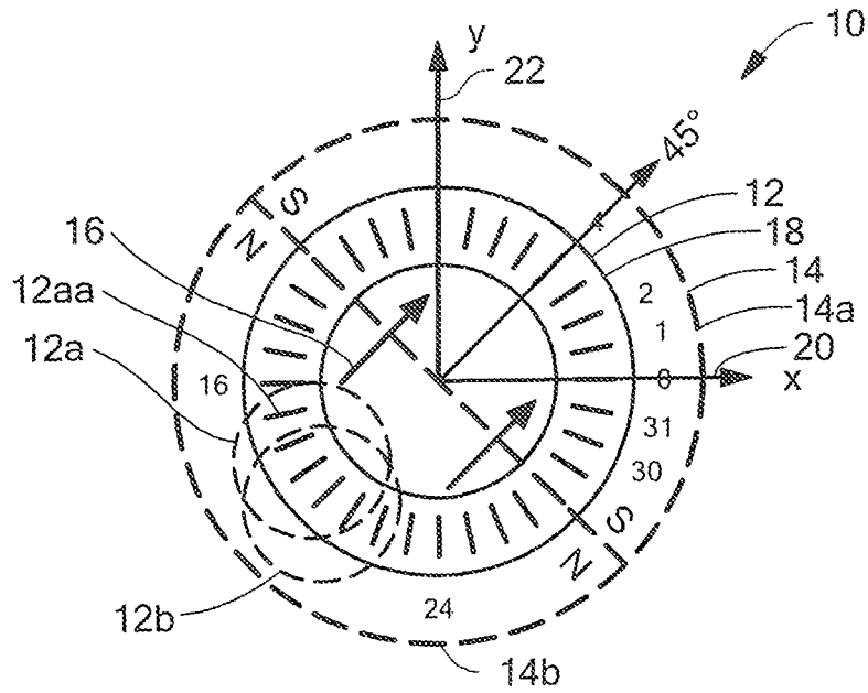
FIG. 1 (PRIOR ART)
