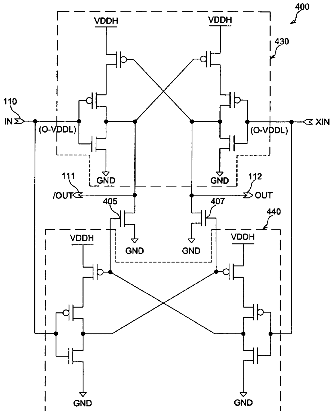
FIG. 4 (PRIOR ART)
