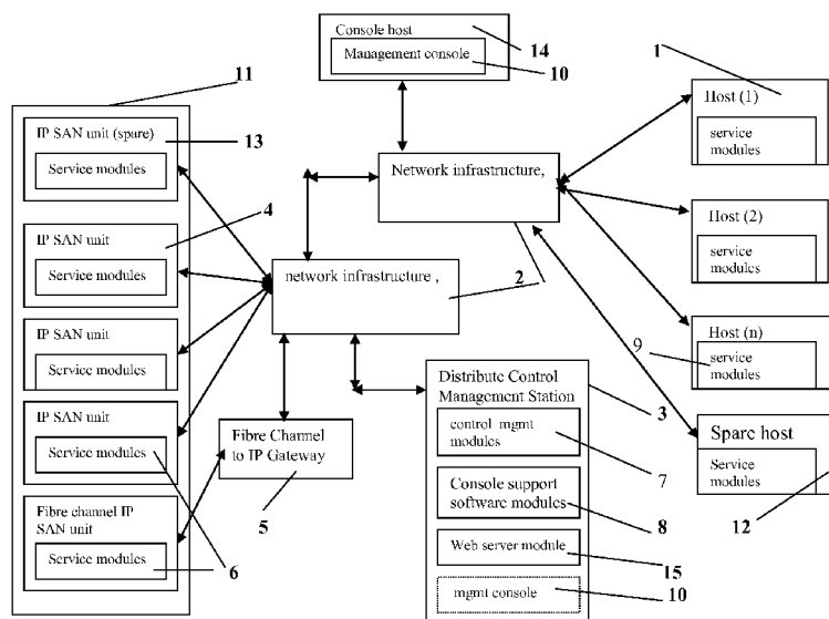
Distributed Virtual SAN Infrastructure
