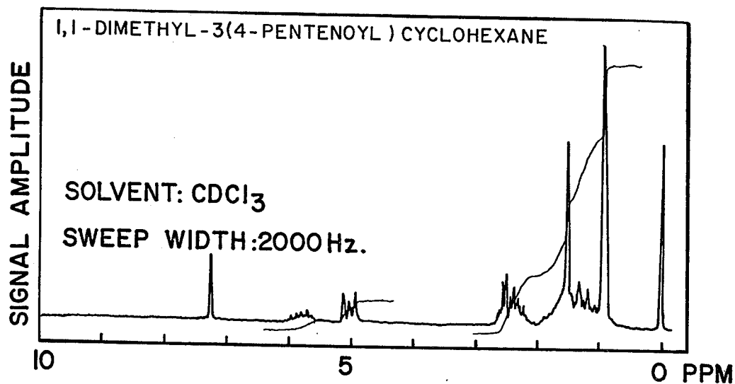
FIG.3 NMR SPECTRUM EXAMPLE I
