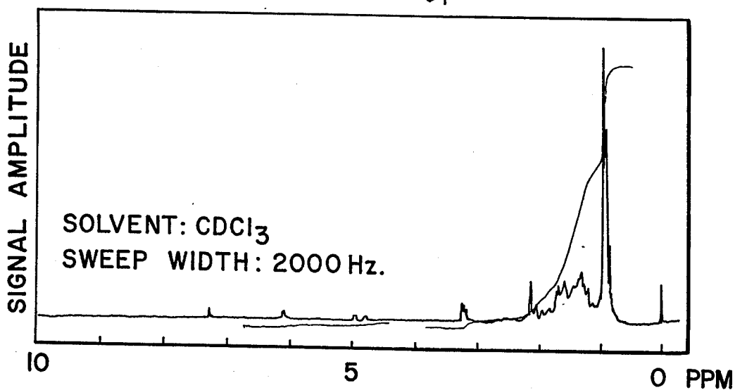
NMR SPECTRUM FOR:
