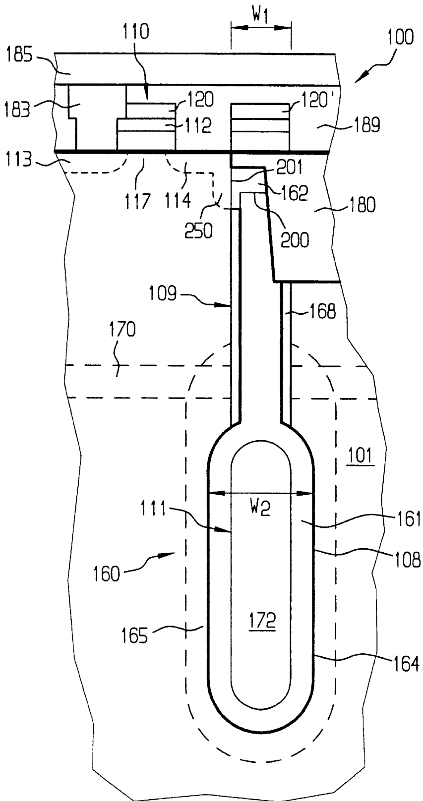
FIG 8 PRIOR ART
