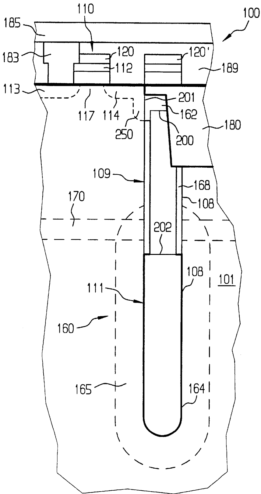
FIG 9 PRIOR ART
