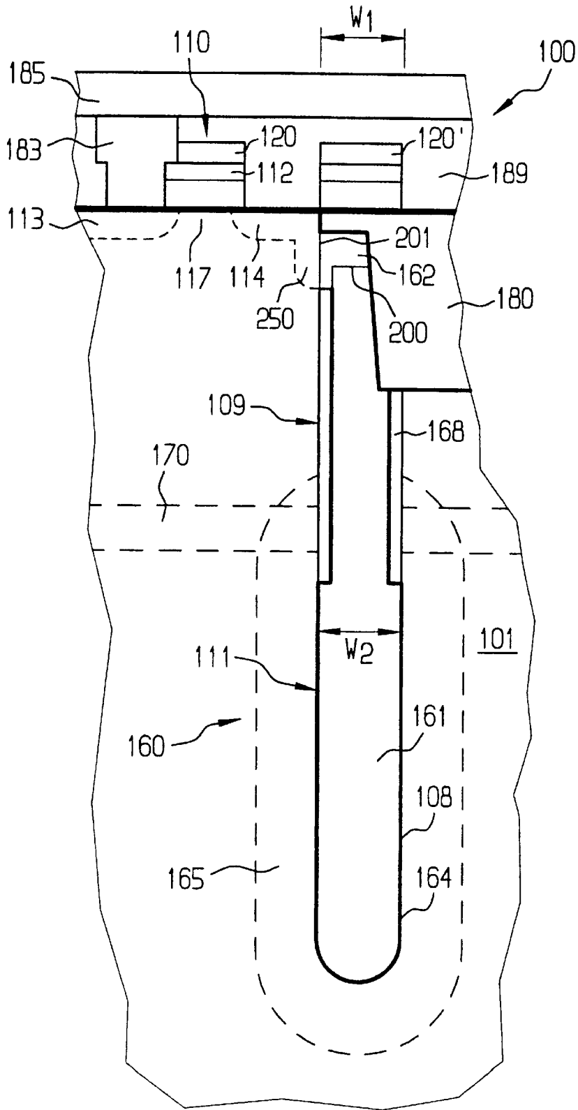
FIG 6 PRIOR ART
