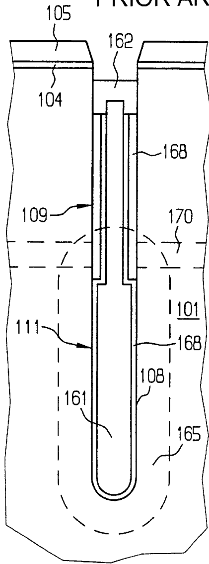
PRIOR ART
