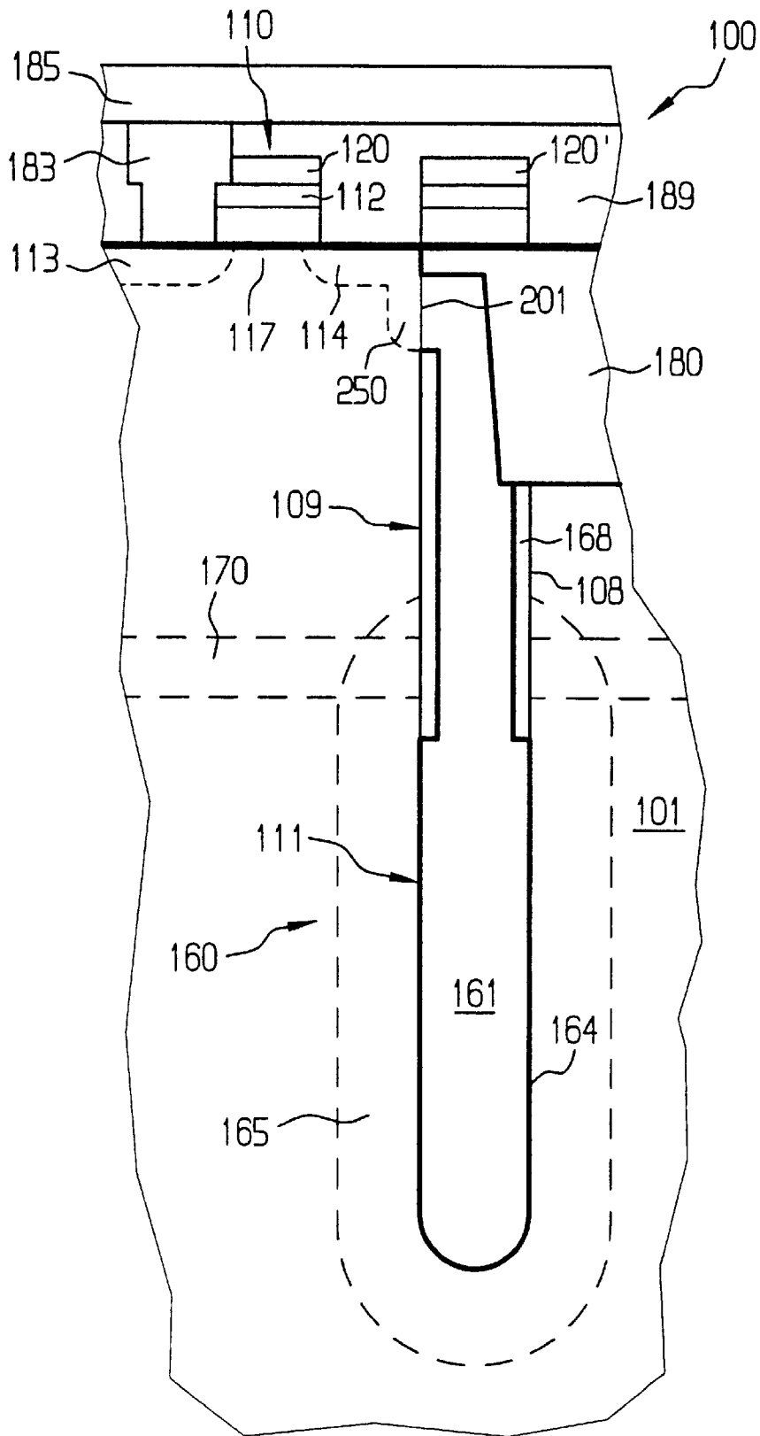
FIG 10 PRIOR ART
