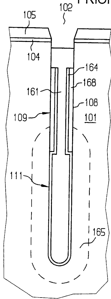
FIG 11d
