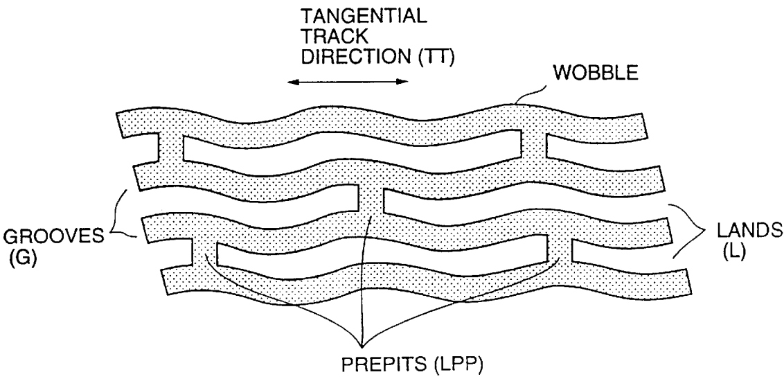
FIG. 10 PRIOR ART
