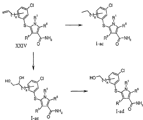
Reaction scheme 11:
