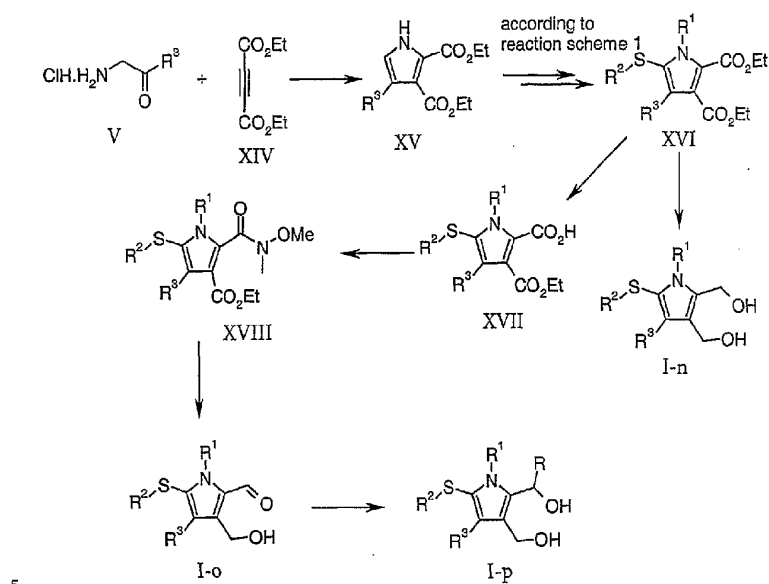
Reaction scheme 6:
