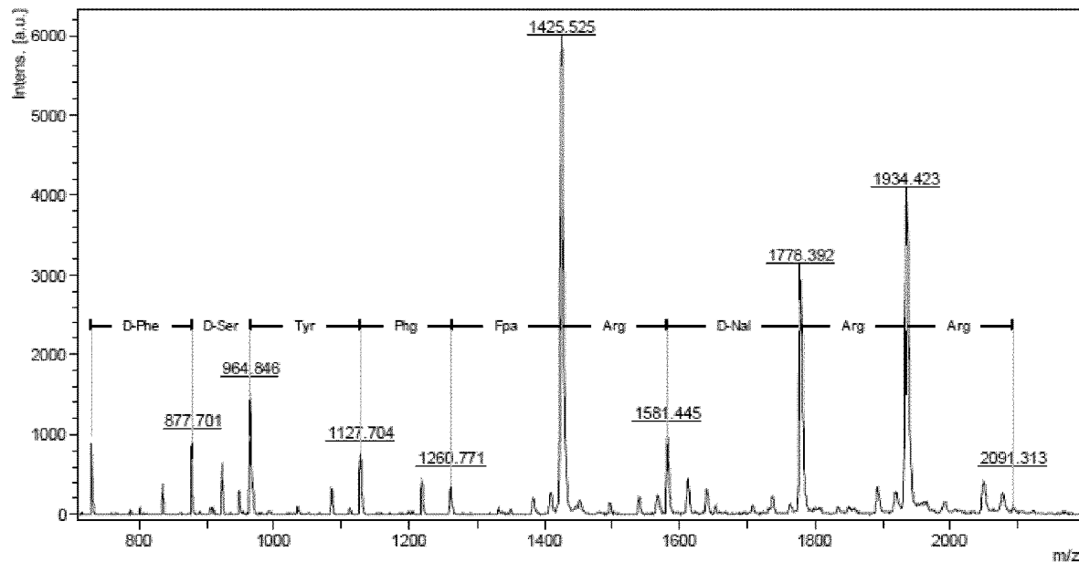
Cyclorasin 8A: cyclo(Arg-Arg-nal-Arg-Fpa-Phg-Tyr-ser-phe-Gln)
