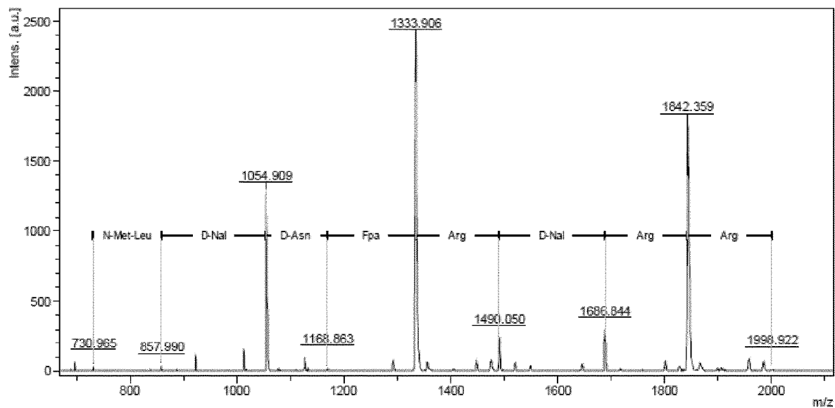
Cyclorasin 3A: cyclo(Arg-Arg-nal-Arg-Fpa-asn-nal-MeLeu-Gln)
