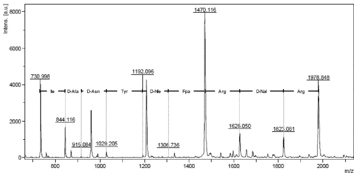
Cyclorasin 10A: cyclo(Arg-Arg-nal-Arg-Fpa-nle-Tyr-asn-ala-Ile-Gln)
