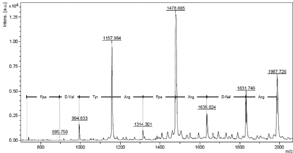
Cyclorasin 7A: cyclo(Arg-Arg-nal-Arg-Fpa-Arg-Tyr-val-Fpa-Gln)
