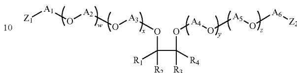
Formula (II)
