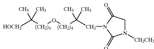
[0447] 1-ethyl-3-[6-(6-hydroxy-5,5-dimethyl-hexyloxy)-2,2-dimethyl-hexyl]-imidazolidine-2,4-dione;
