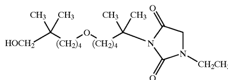
[0446] 1-ethyl-3-[5-(6-hydroxy-5,5-dimethyl-hexyloxy)-1,1-dimethyl-pentyl]-imidazolidine-2,4-dione;
