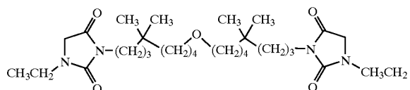
[0486] 3-[7-(8-(3-ethyl-2,5-dioxoimidazolidin-1-yl)-5,5-dimethyl-octyloxy)-3,3-dimethyl-heptyl]-1-ethyl-imidazolidine-2,4-dione;
