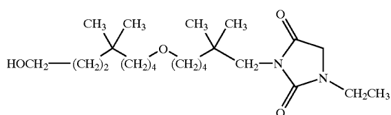
[0451] 1-ethyl-3-[6-(8-hydroxy-5,5-dimethyl-octyloxy)-2,2-dimethyl-hexyl]-imidazolidine-2,4-dione;
