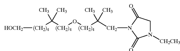
[0458] 1-ethyl-3-[6-(10-hydroxy-5,5-dimethyl-decyloxy)-2,2-dimethyl-hexyl]-imidazolidine-2,4-dione;
