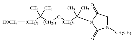
[0453] 1-ethyl-3-[5-(9-hydroxy-5,5-dimethyl-nonyloxy)-1,1-dimethyl-pentyl]-imidazolidine-2,4-dione;
