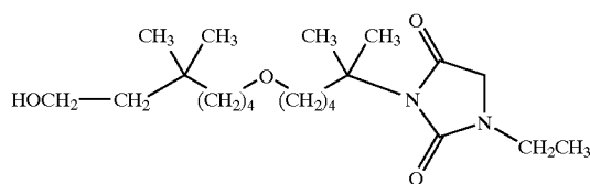
[0447] 1-ethyl-3-[6-(6-hydroxy-5,5-dimethyl-hexyloxy)-2,2-dimethyl-hexyl]-imidazolidine-2,4-dione;
