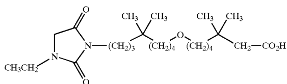
[0470] 7-[8-(3-ethyl-2,5-dioxo-imidazolidin-1-yl)-5,5-dimethyl-octyloxy]-3,3-dimethyl-heptanoic acid;
