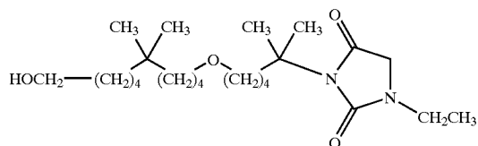
[0457] 1-ethyl-3-[5-(10-hydroxy-5,5-dimethyl-decyloxy)-1,1-dimethyl-pentyl]-imidazolidine-2,4-dione;
