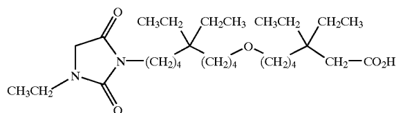
[0315] 7-[5,5-diethyl-9-(3-ethyl-2,5-dioxo-imidazolidin-1-yl)-nonyloxy]-3,3-diethyl-heptanoic acid;
