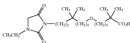
[0466] 6-[7-(3-ethyl-2,5-dioxo-imidazolidin-1-yl)-5,5-dimethyl-heptyloxy]-2,2-dimethyl-hexanoic acid;
