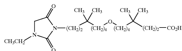
[0468] 8-[7-(3-ethyl-2,5-dioxo-imidazolidin-1-yl)-5,5-dimethyl-heptyloxy]-4,4-dimethyl-octanoic acid;
