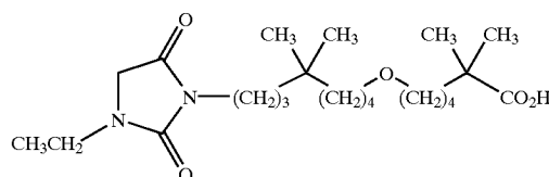
[0469] 6-[8-(3-ethyl-2,5-dioxo-imidazolidin-1-yl)-5,5-dimethyl-octyloxy]-2,2-dimethyl-hexanoic acid;
