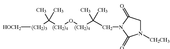
[0454] 1-ethyl-3-[6-(9-hydroxy-5,5-dimethyl-nonyloxy)-2,2-dimethyl-hexyl]-imidazolidine-2,4-dione;
