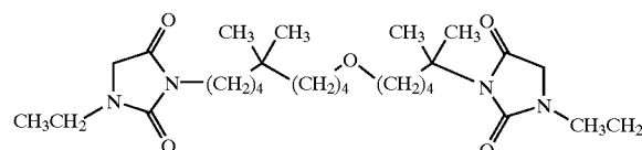
[0487] 3-[8-(8-(3-ethyl-2,5-dioxoimidazolidin-1-yl)-5,5-dimethyl-octyloxy)-4,4-dimethyl-octyl]-1-ethyl-imidazolidine-2,4-dione;
