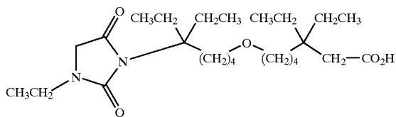
[0303] 2,2-diethyl-6-[5-ethyl-5-(3-ethyl-2,5-dioxo-imidazolidin-1-yl)-heptyloxy]-hexanoic acid;
