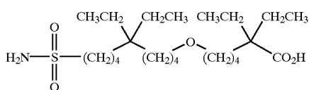
[0267] 6-(5,5-diethyl-9-sulfamoyl-nonyloxy)-2,2-diethyl-hexanoic acid;
