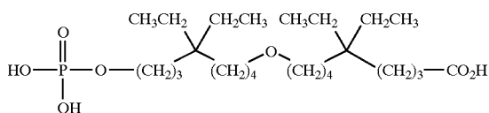
[0219] 9-(5,5-diethyl-8-phosphonooxy-octyloxy)-5,5-diethyl-nonanoic acid;
