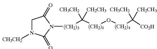
[0310] 6-[5,5-diethyl-8-(3-ethyl-2,5-dioxo-imidazolidin-1-yl)-octyloxy]-2,2-diethyl-hexanoic acid;
