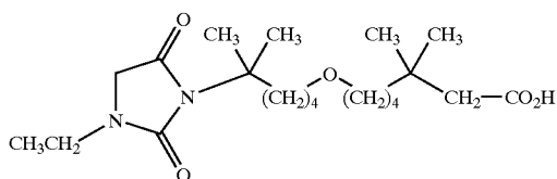
[0463] 7-[5-(3-ethyl-2,5-dioxo-imidazolidin-1-yl)-5-methyl-hexyloxy]-3,3-dimethyl-heptanoic acid;
