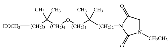
[0455] 1-ethyl-3-[7-(9-hydroxy-5,5-dimethyl-nonyloxy)-3,3-dimethyl-heptyl]-imidazolidine-2,4-dione;
