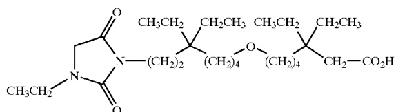
[0308] 7-[5,5-diethyl-7-(3-ethyl-2,5-dioxo-imidazolidin-1-yl)-heptyloxy]-3,3-diethyl-heptanoic acid;
