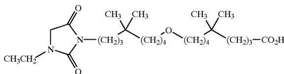
[0471] 8-[8-(3-ethyl-2,5-dioxo-imidazolidin-1-yl)-5,5-dimethyl-octyloxy]-4,4-dimethyl-octanoic acid;
