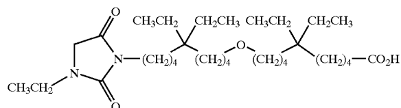
[0318] 10-[5,5-diethyl-9-(3-ethyl-2,5-dioxo-imidazolidin-1-yl)-nonyloxy]-6,6-diethyl-decanoic acid;
