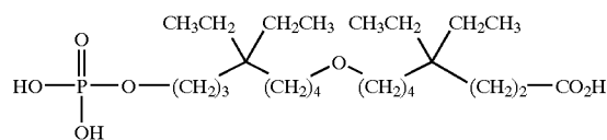
[0218] 8-(5,5-diethyl-8-phosphonooxy-octyloxy)-4,4-diethyl-octanoic acid;
