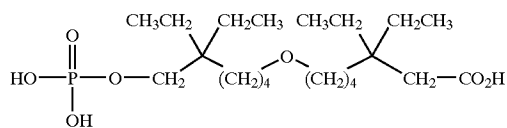
[0212] 3,3-diethyl-7-(5-ethyl-5-phosphonooxymethyl-heptyloxy)-heptanoic acid;
