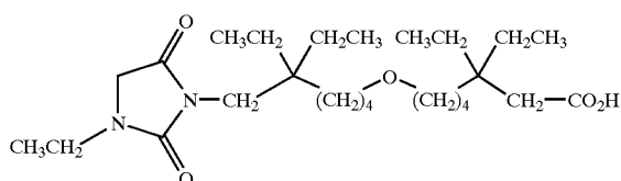
[0306] 3-diethyl-7-[5-ethyl-5-(3-ethyl-2,5-dioxo-imidazolidin-1-ylmethyl)-heptyloxy]-heptanoic acid;
