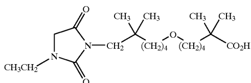
[0464] 6-[6-(3-ethyl-2,5-dioxo-imidazolidin-1-yl)-5,5-dimethyl-hexyloxy]-2,2-dimethyl-hexanoic acid;
