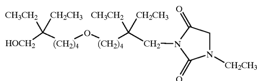
[0287] 3-[1,1-diethyl-5-(5-ethyl-5-hydroxymethyl-heptyloxy)-pentyl]-1-ethyl-imidazolidine-2,4-dione;
