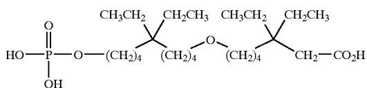
[0221] 7-(5,5-diethyl-9-phosphonooxy-nonyloxy)-3,2-diethyl-heptanoic acid;
