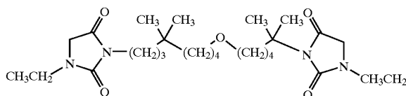
[0484] 3-[5-(8-(3-ethyl-2,5-dioxoimidazolidin-1-yl)-5,5-dimethyl-octyloxy)-1,1-dimethyl-pentyl]-1-ethyl-imidazolidine-2,4-dione;
