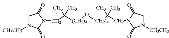
[0480] 3-[6-(6-(3-ethyl-2,5-dioxoimidazolidin-1-yl)-5,5-dimethyl-hexyloxy)-2,2-dimethyl-hexyl]-1-ethyl-imidazolidine-2,4-dione;
