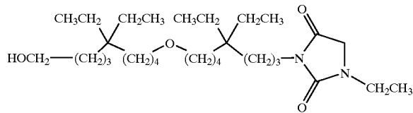
[0297] 3-[8-(5,5-diethyl-9-hydroxy-nonyloxy)-4,4-diethyl-octyl]-1-ethyl-imidazolidine-2,4-dione;
