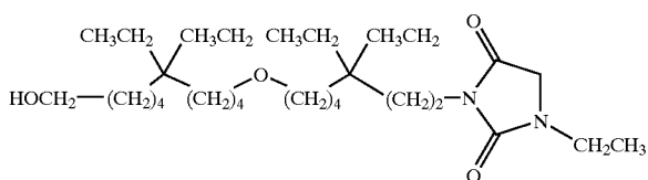
[0300] 3-[7-(5,5-diethyl-10-hydroxy-decyloxy)-3,3-diethyl-heptyl]-1-ethyl-imidazolidine-2,4-dione;
