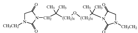
[0479] 3-[5-(6-(3-ethyl-2,5-dioxo-imidazolidin-1-yl)-5,5-dimethyl-hexyloxy)-1,1-dimethyl-pentyl]-1-ethyl-imidazolidine-2,4-dione;
