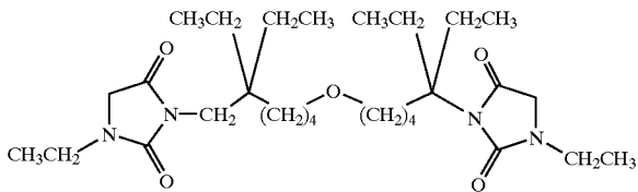
[0320] 3-[5-(5-(3-ethyl-2,5-dioxo-imidazolidin-1-yl)-methyl-5-ethyl-heptyloxy)-1,1-diethyl-pentyl]-1-ethyl-imidazolidine-2,4-dione;
