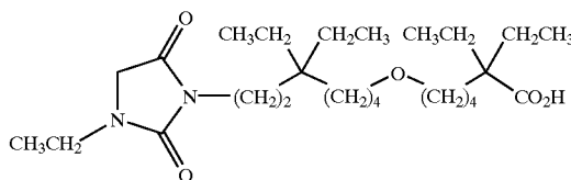
[0307] 6-[5,5-diethyl-7-(3-ethyl-2,5-dioxo-imidazolidin-1-yl)-heptyloxy]-2,2-diethyl-hexanoic acid;
