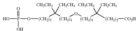
[0215] 8-(5,5-diethyl-7-phosphonooxy-heptyloxy)-4,3-diethyl-octanoic acid;
