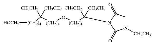
[0298] 3-[5-(5,5-diethyl-10-hydroxy-decyloxy)-1,1-diethyl-pentyl]-1-ethyl-imidazolidine-2,4-dione;
