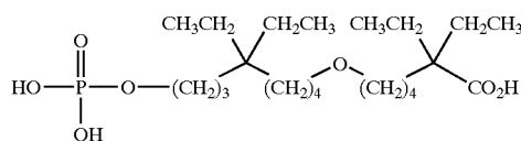
[0216] 6-(5,5-diethyl-8-phosphonooxy-octyloxy)-2,2-diethyl-hexanoic acid;
