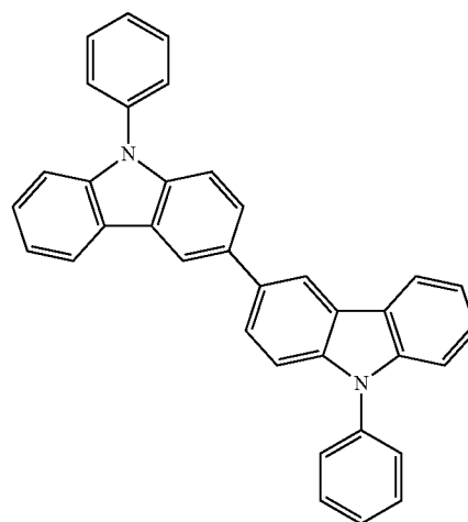
PCCP
