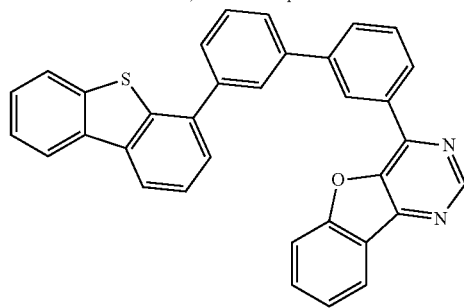
4mDBtBP2Bfpm-II
