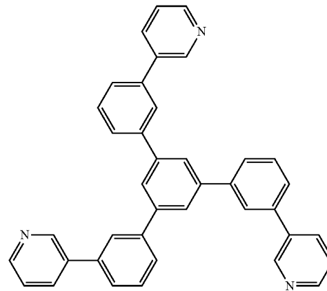
TmPyPB
