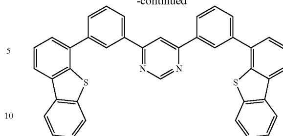
4,6mDBT2Pm-II
