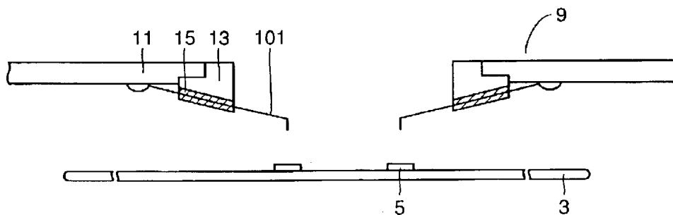
FIG. 18 PRIOR ART
