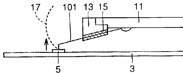
FIG. 19 PRIOR ART
