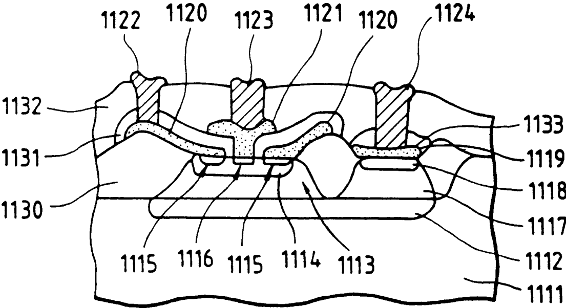
FIG. 12 (PRIOR ART)
