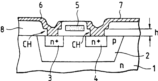
FIG. 11C (PRIOR ART)
