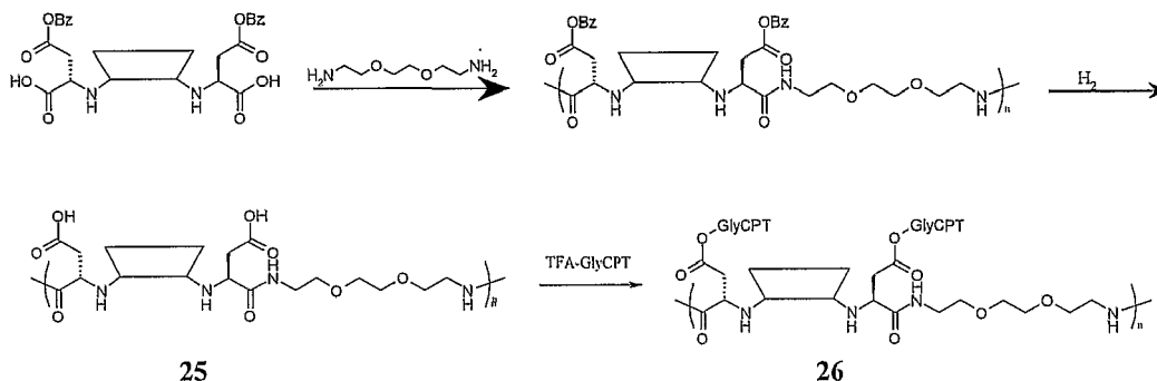
Scheme XXXI
