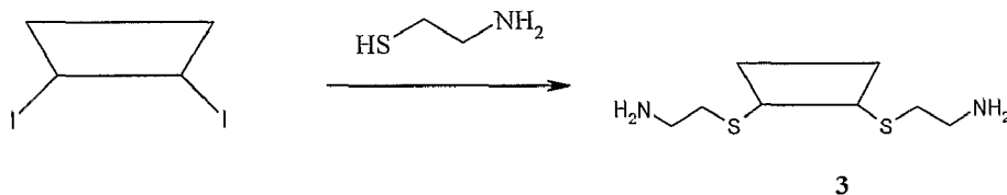
Scheme XVII
