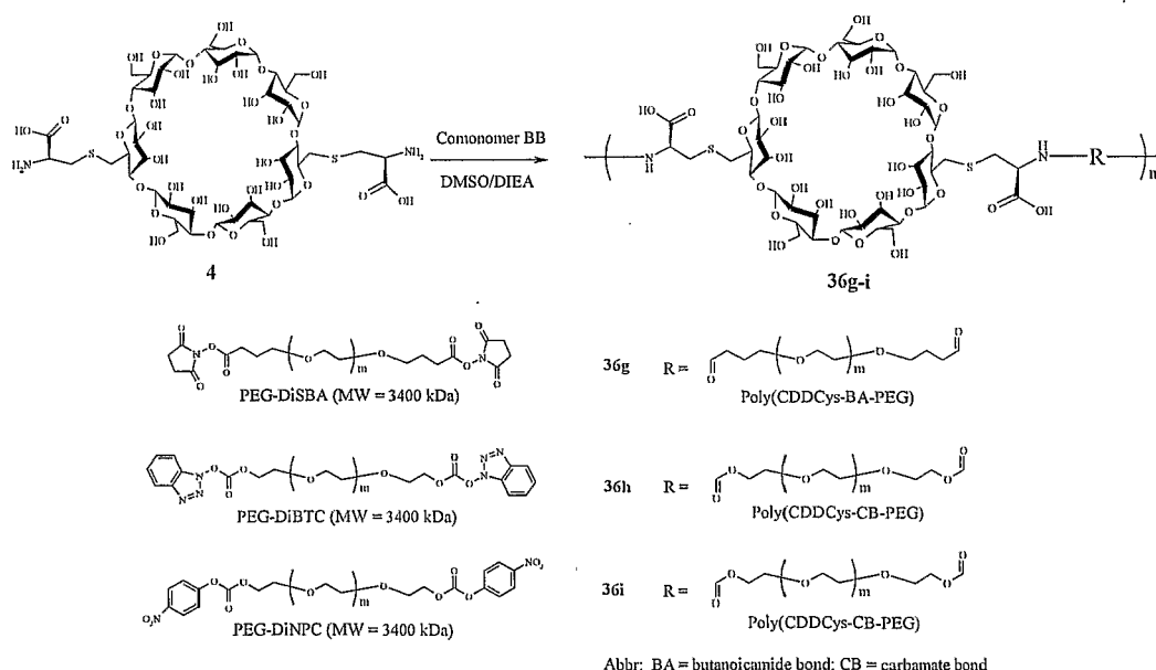
Scheme XXXVIIIb
