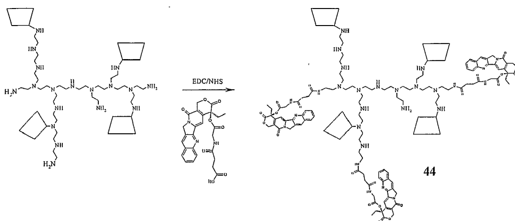
Scheme XXXXV
