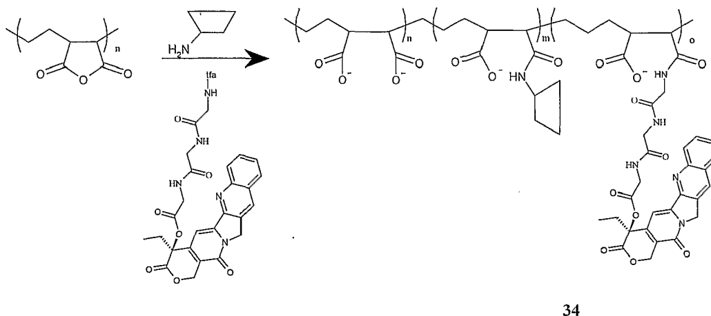
Scheme XXXVI
