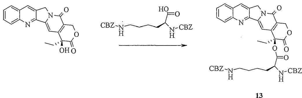
Scheme XXVII
