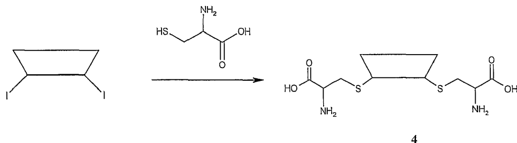
Scheme XVIII
