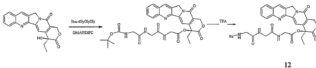
Scheme XXVI
