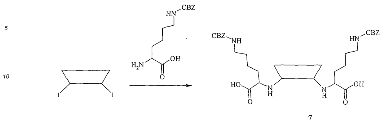
Scheme XXI
