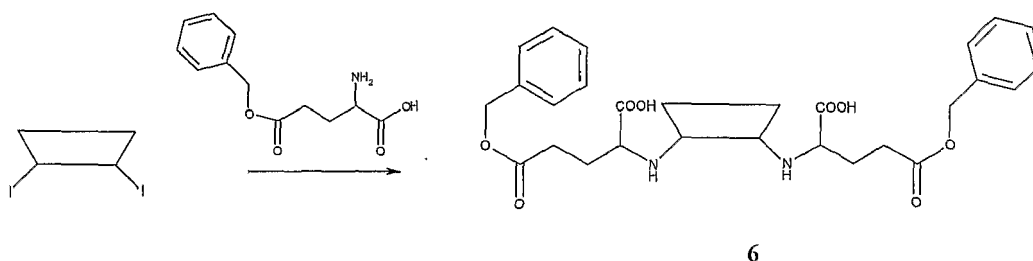
Scheme XX
