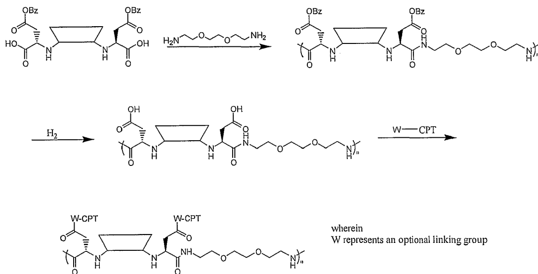
Scheme V
