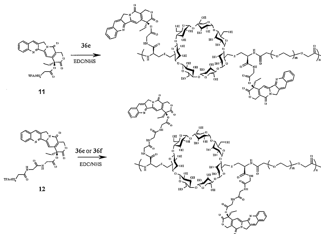
Scheme XXXIX
