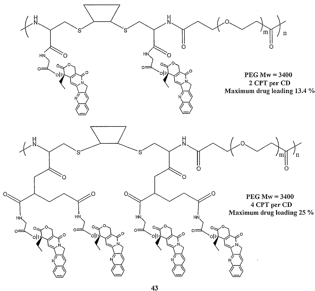
Scheme XXXXIII
