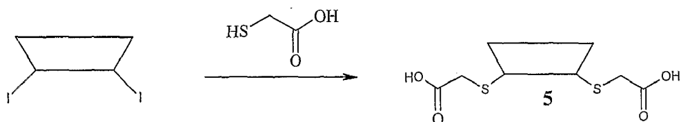
Scheme XIX
