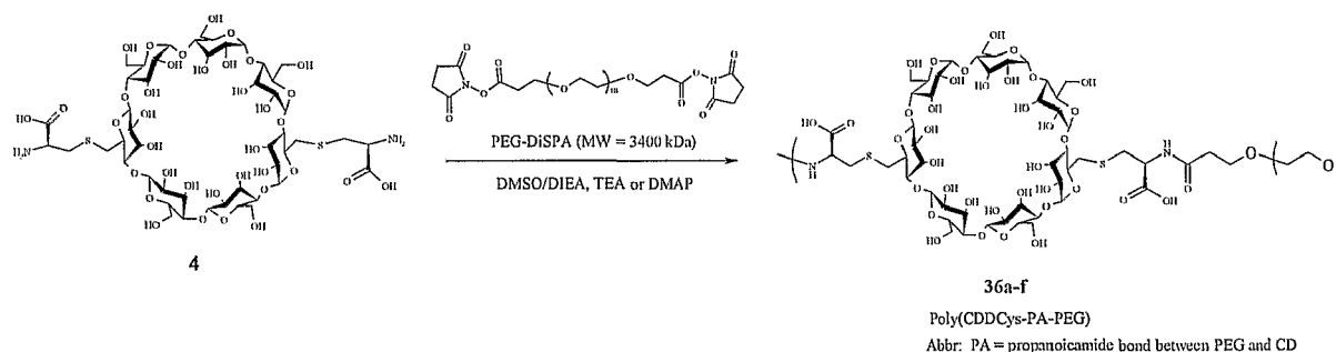
Scheme XXXVIIIb
