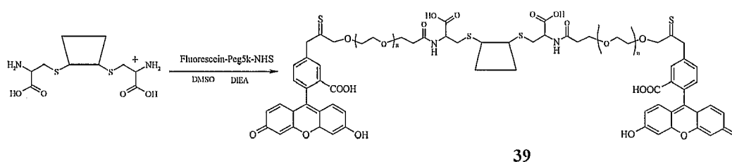
Scheme XXXX
