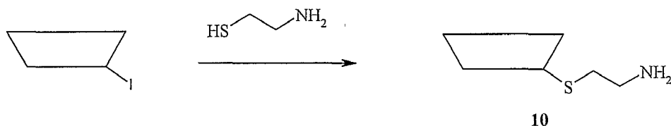
Scheme XXIV
