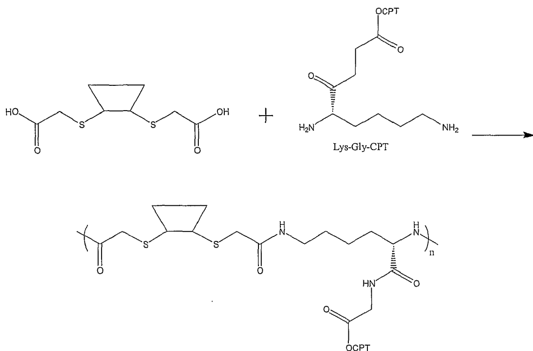
Scheme VIII
