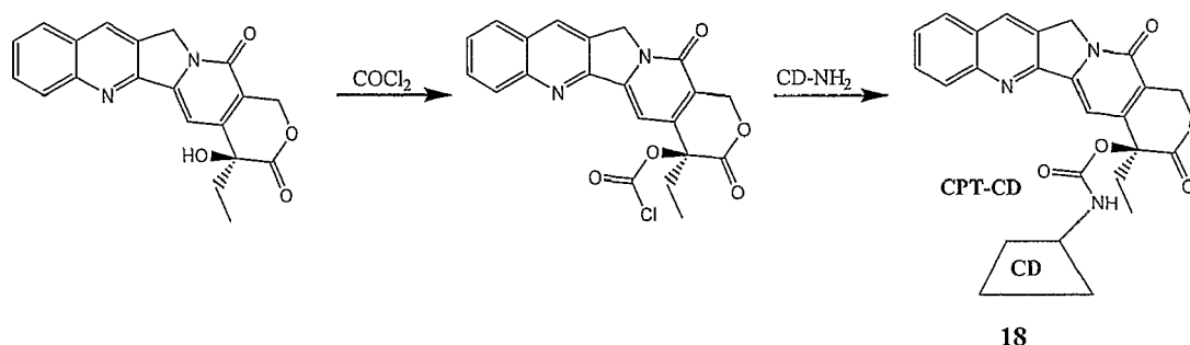
Scheme XXVIII
