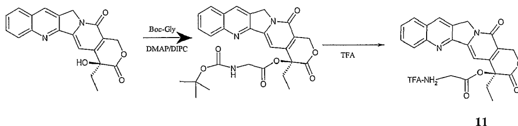
Scheme XXV
