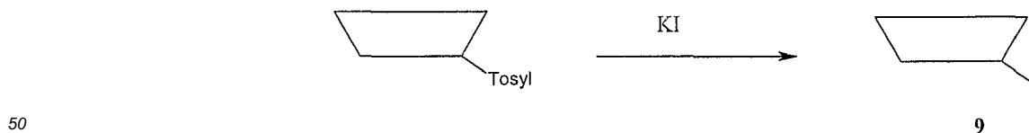
Scheme XXIII
