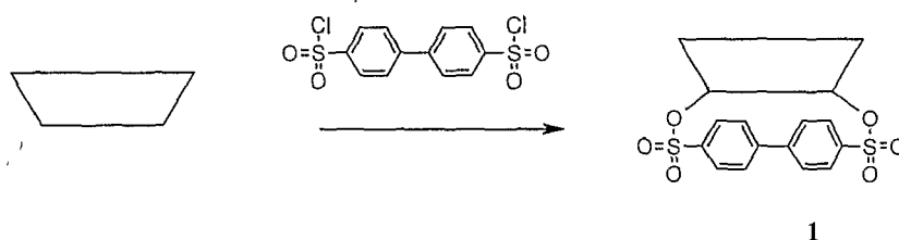
Scheme XV
