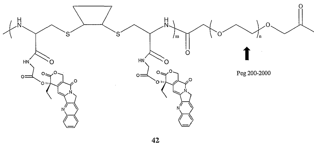
Scheme XXXXII
