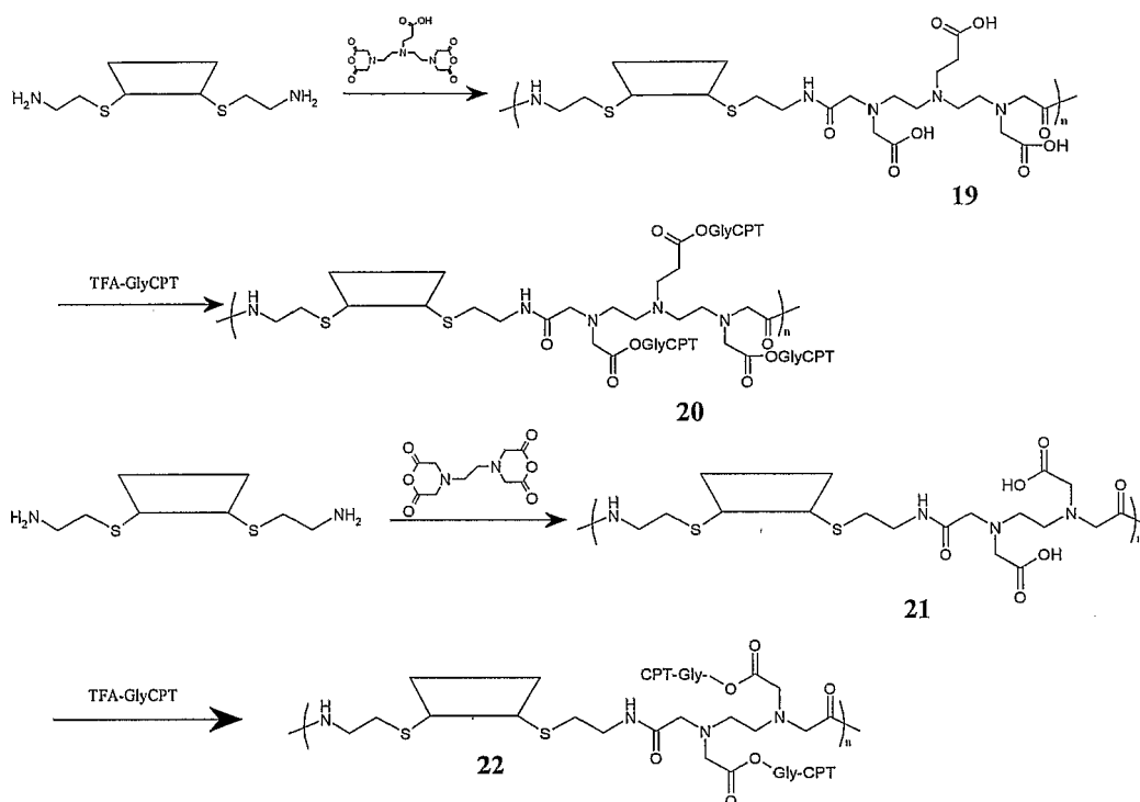
Scheme XXIX
