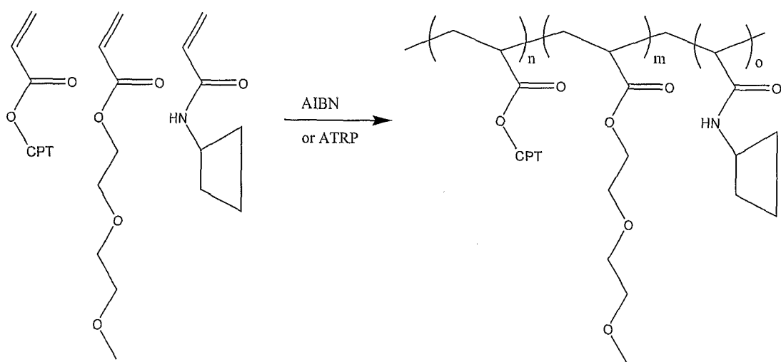
Scheme XI
