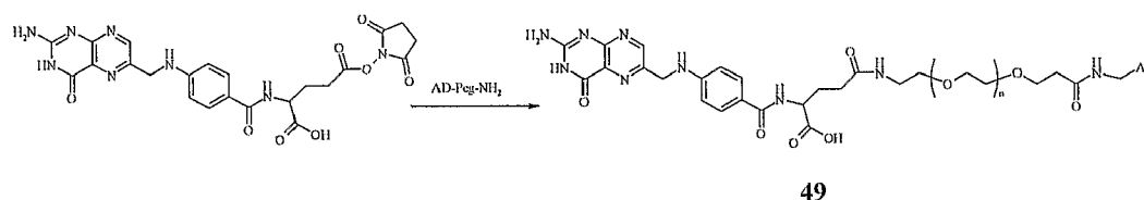
Scheme L
