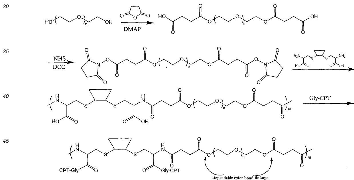
Scheme XIV
