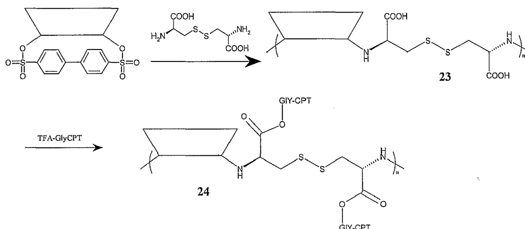
Scheme XXX
