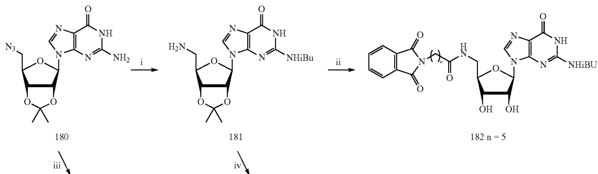
Scheme 9 a
