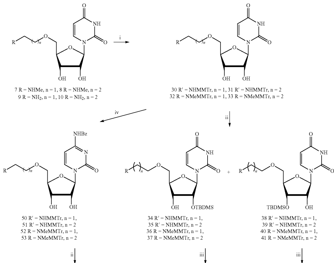
Scheme 2 a
