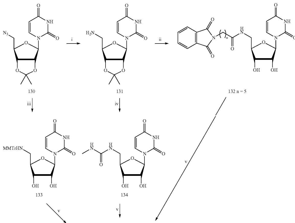
Scheme 6 a
