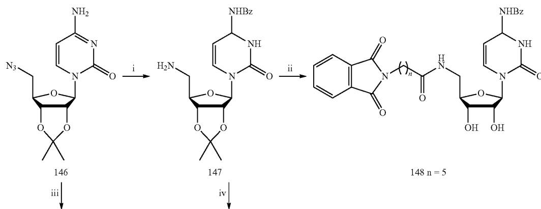
Scheme 7 a
