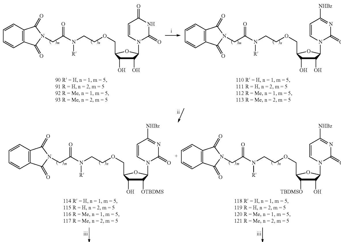
Scheme 5 a
