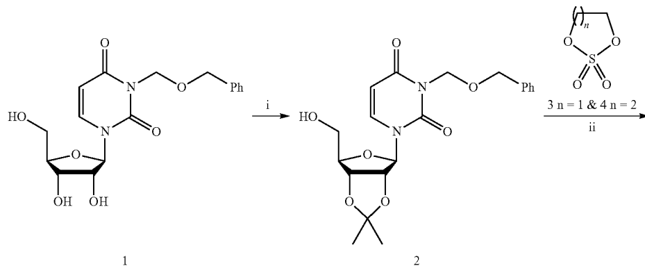
Scheme 1 a
