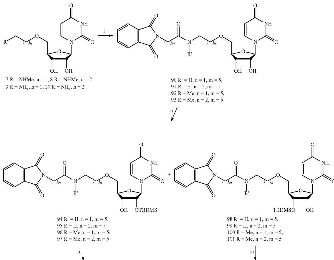
Scheme 4 a
