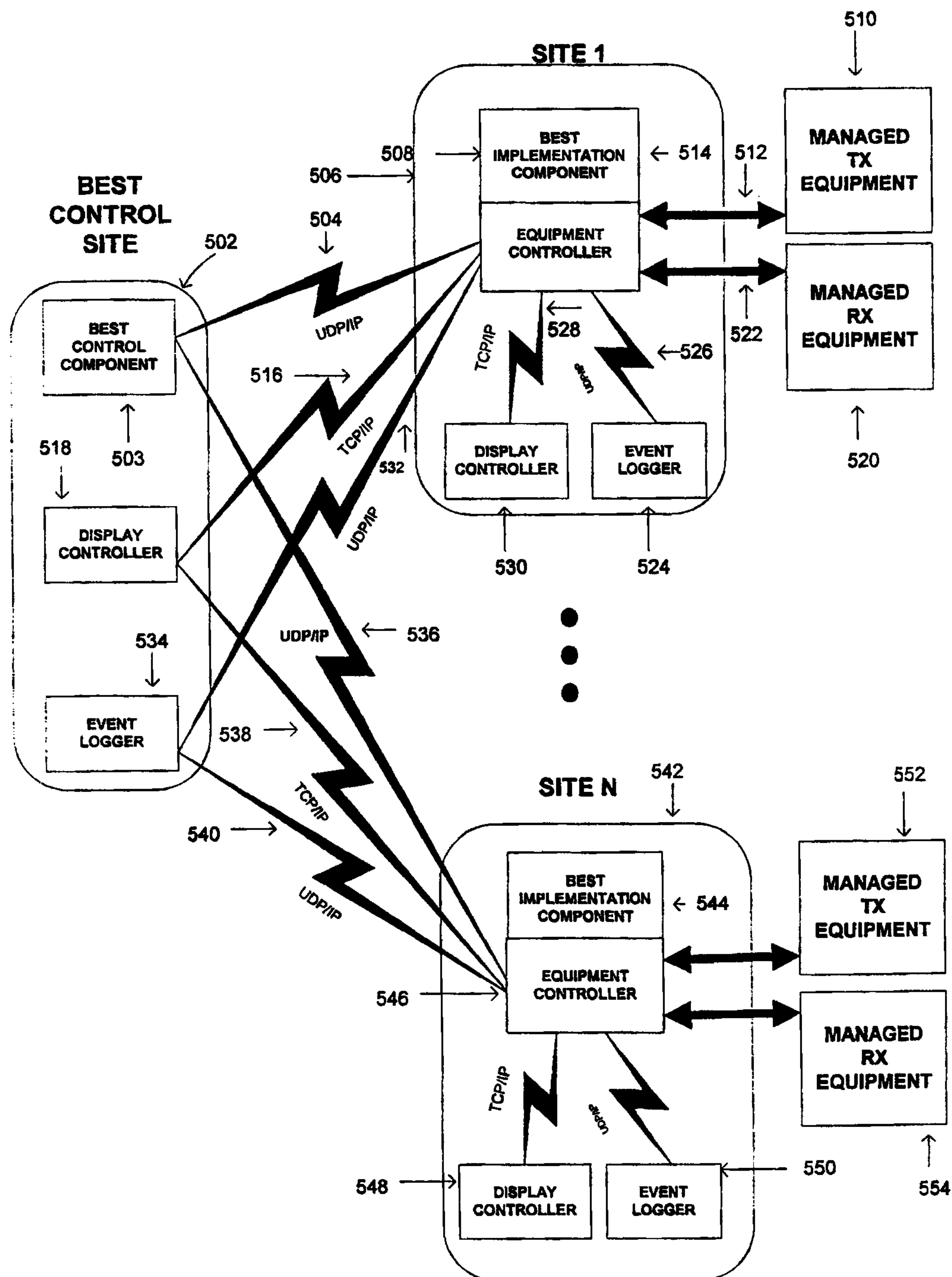
Figure 5 DISTRIBUTED SOFTWARE COMPONENTS
