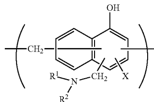
[Chemical Formula 4]
