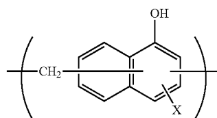
[Chemical Formula 4]
