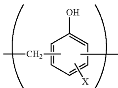
[Chemical Formula 1]
