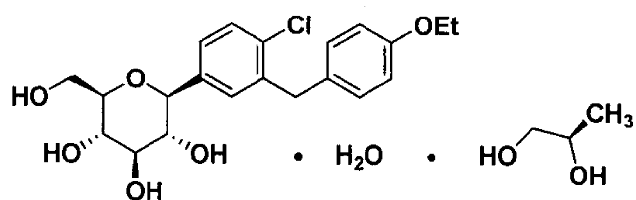
Ib (form SD-3, (R)-PG)
