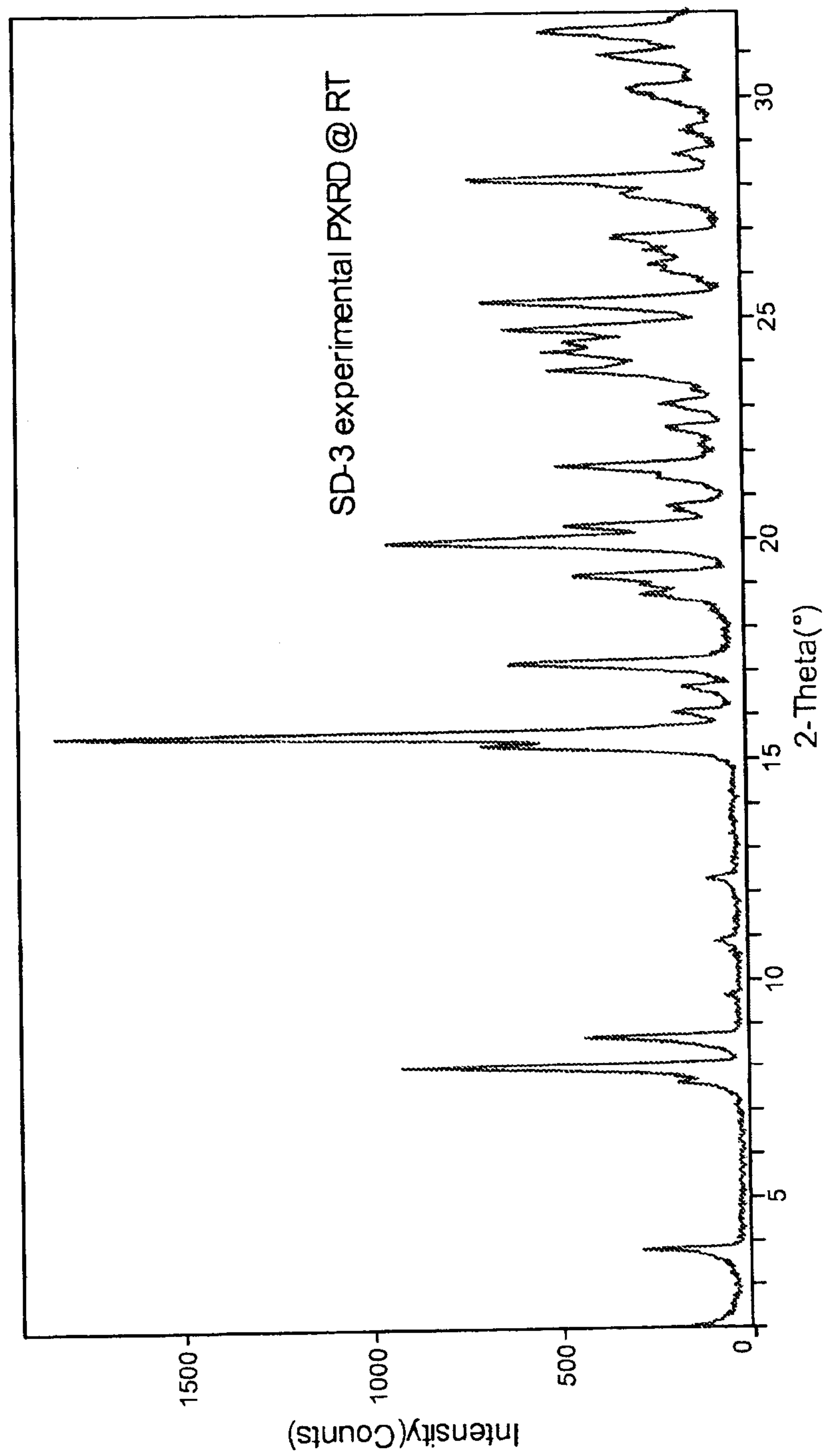
FIG. 2 Powder X-ray diffraction patterns of (R)-PG Ib
