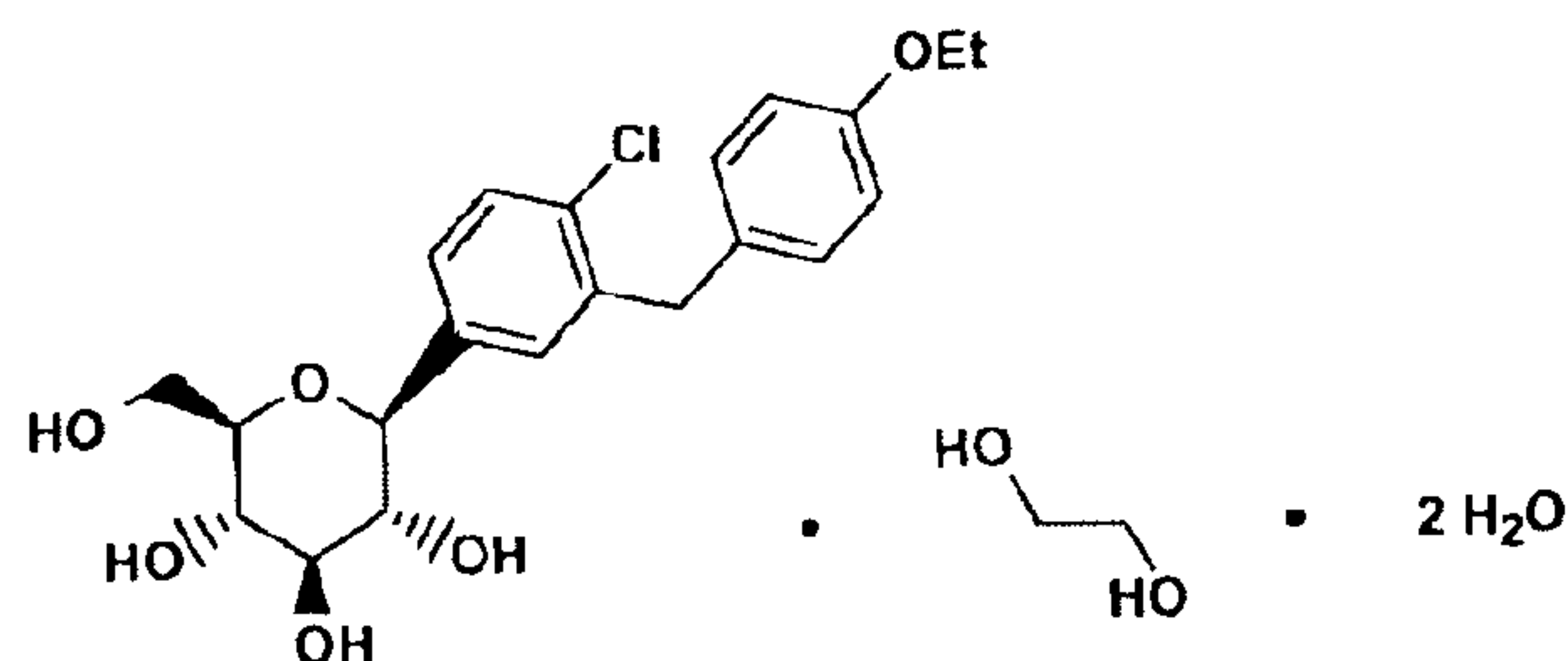
Ethylene Glycol Form SB-1
