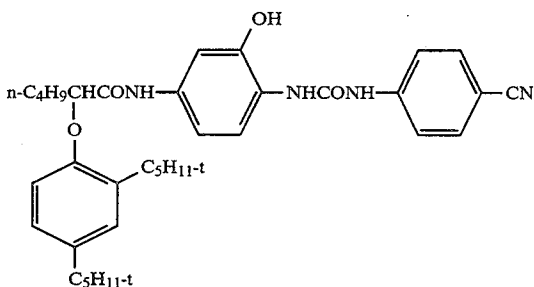
Typical Dye Image-Forming Coupler Compounds
