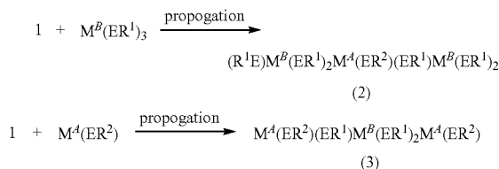
REACTION SCHEME 2:
