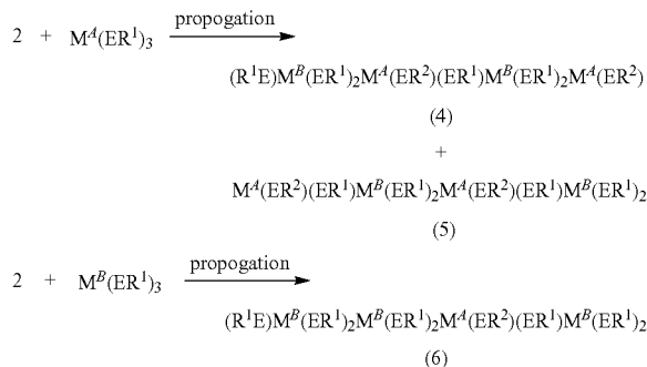
REACTION SCHEME 3:
