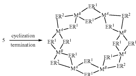
REACTION SCHEME 7:
