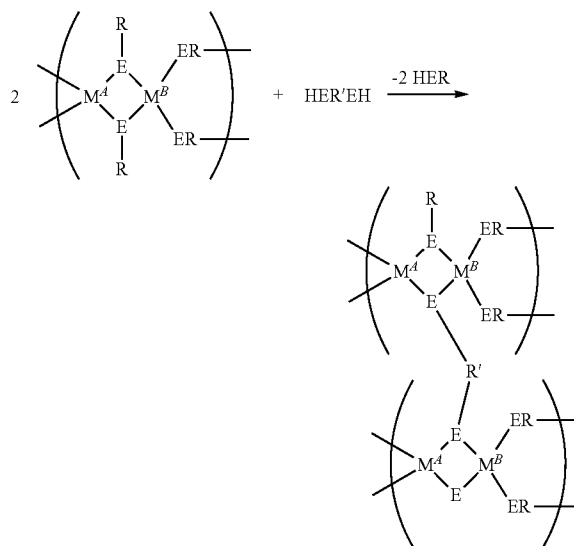
REACTION SCHEME 14
