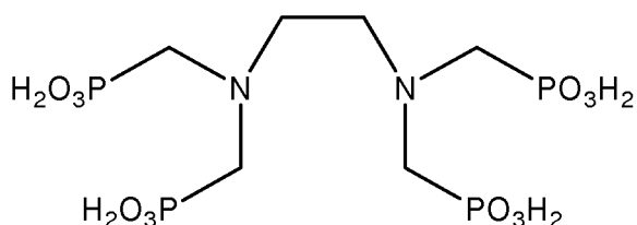
EDTMP
