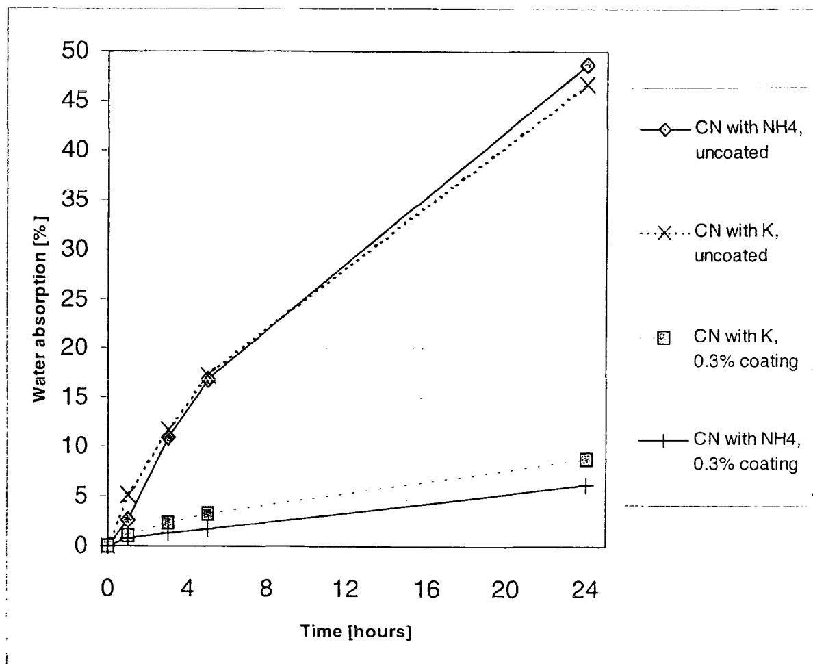
Figure 1: Water absorption at 25 °C and 70% RH.
