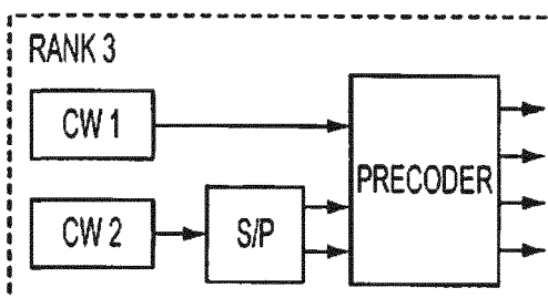
FIG. 5C PRIOR ART
