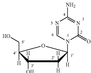
Figure 1: Structure of Decitabine
