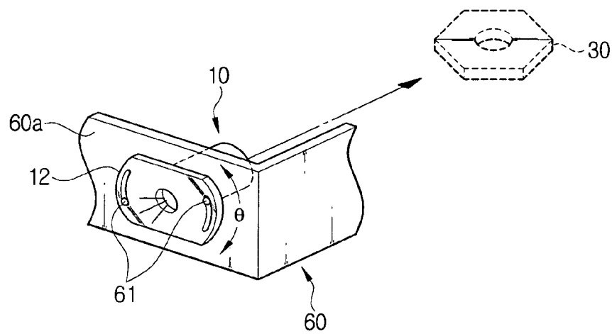
FIG. 2 (PRIOR ART)
