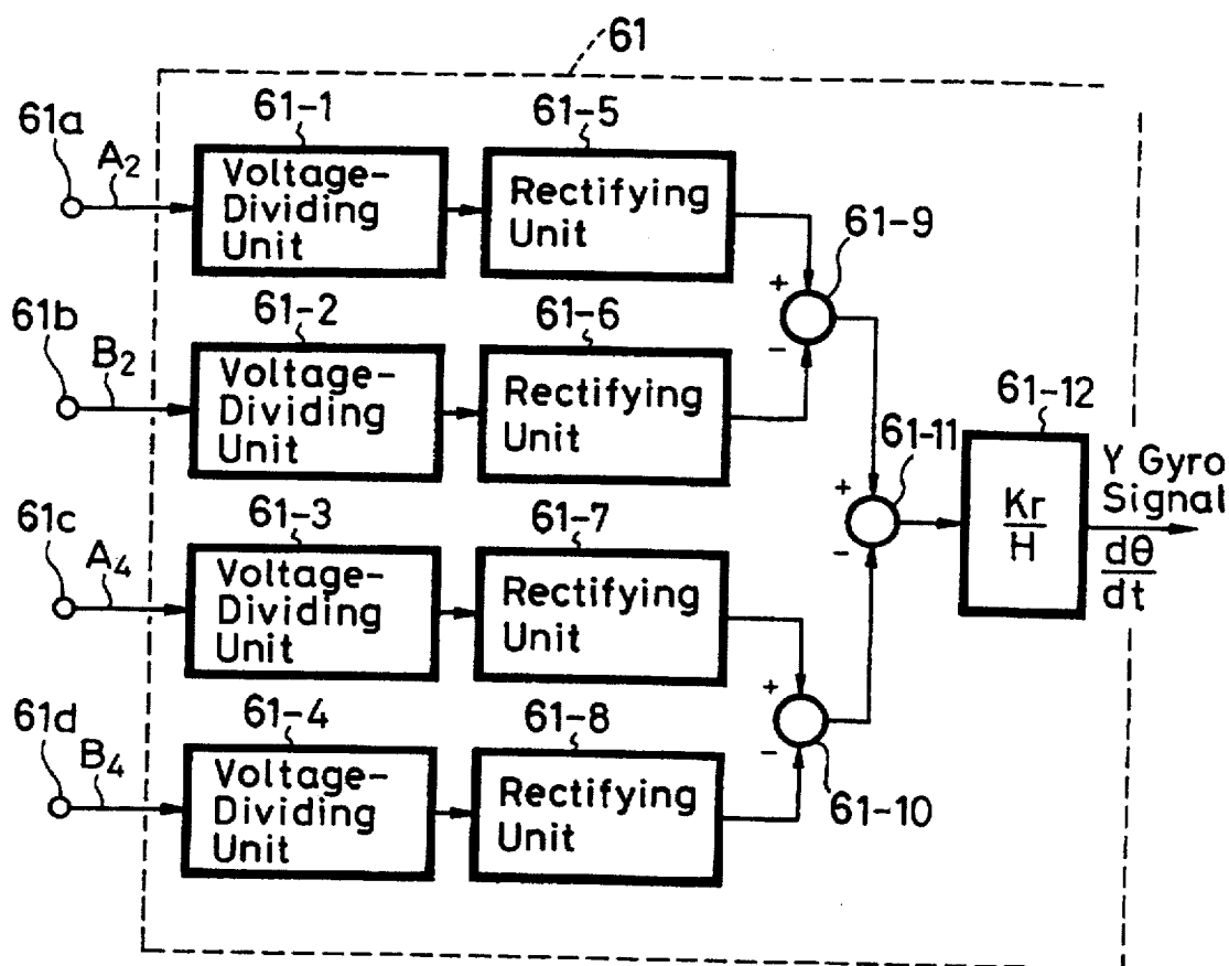
FIG. 6A (RELATED ART)
