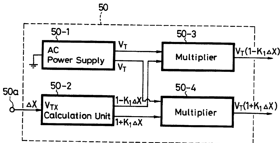
FIG. 4B (RELATED ART)
