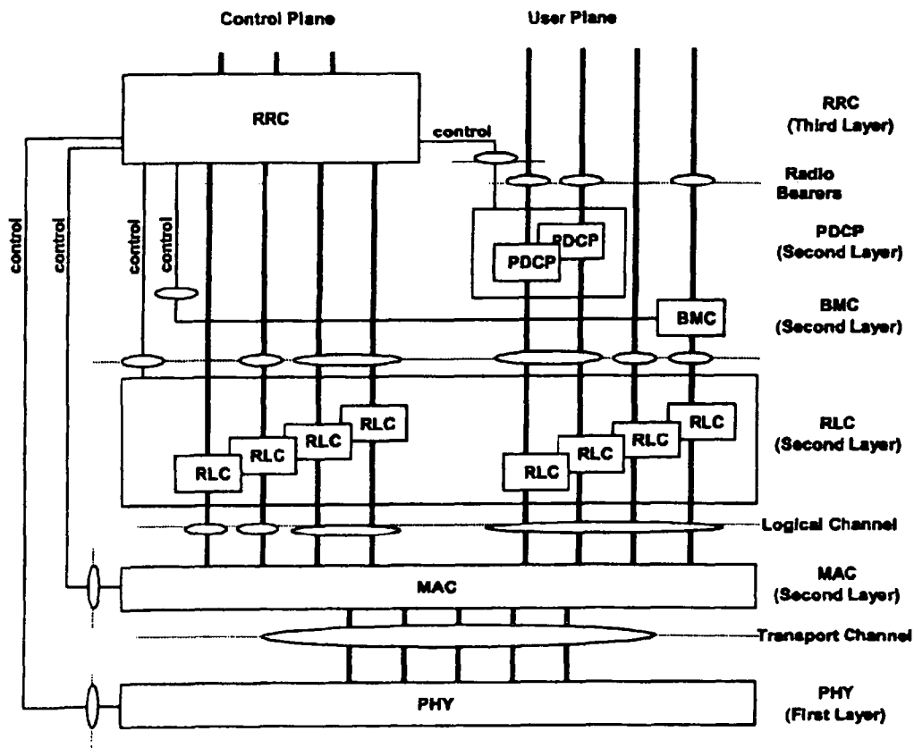
FIG.2 BACKGROUND ART
