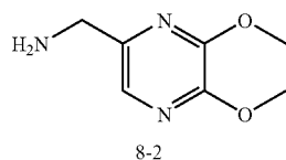
2,3-dimethoxy-5-aminomethylpyrazine (8-2)
