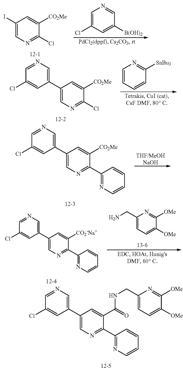
Methyl 5',6-dichloro-3,3'-bipyridine-5-carboxylate (12-5)
