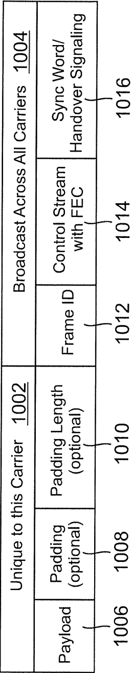
Carrier Framing Structure:
