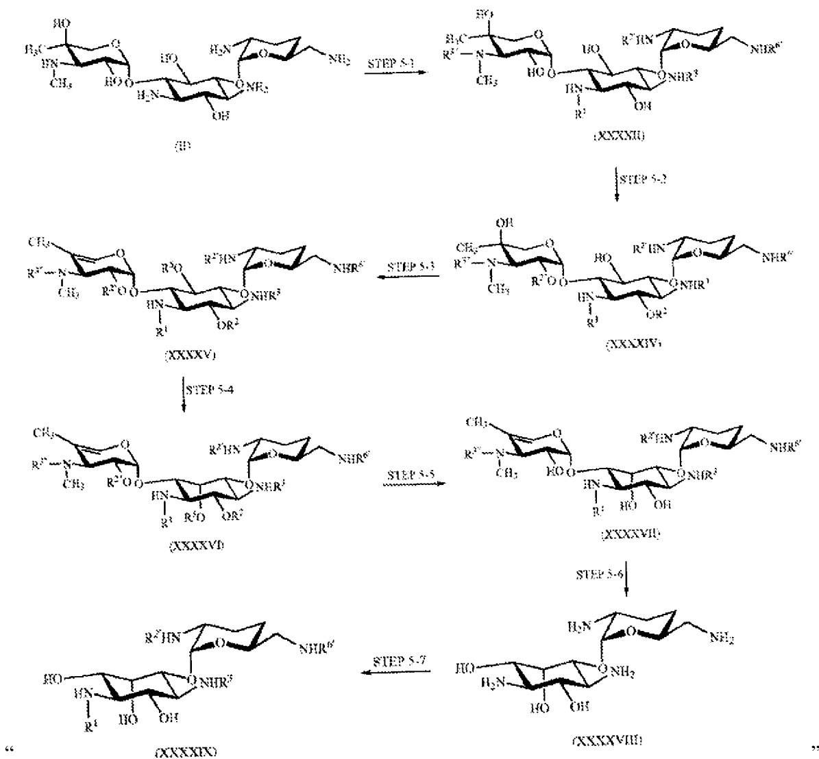
Scheme 10
