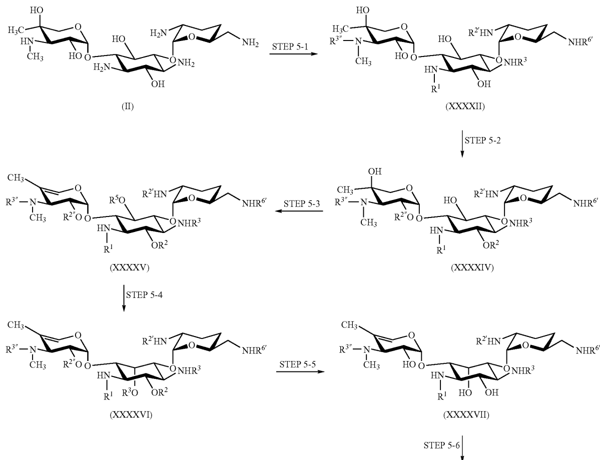
Scheme 10
