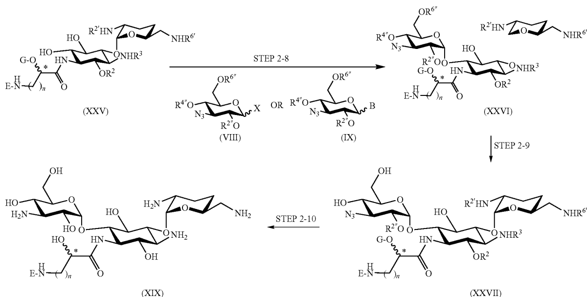
[Chemical formula 30]
