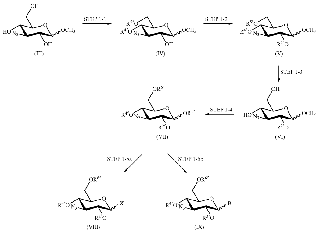
[Chemical formula 24]
