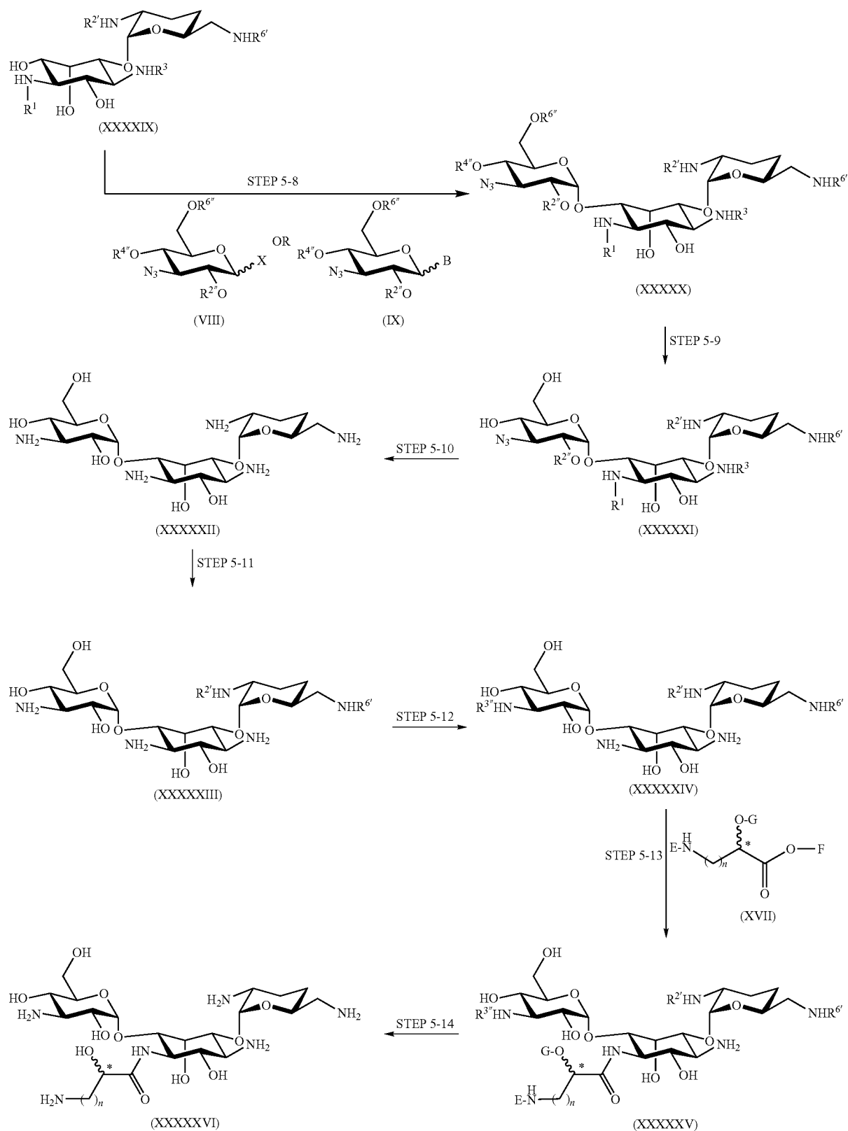
Scheme 11
