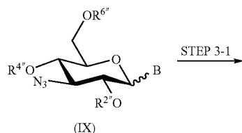
Scheme 6
