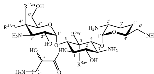
[Chemical formula 2]
