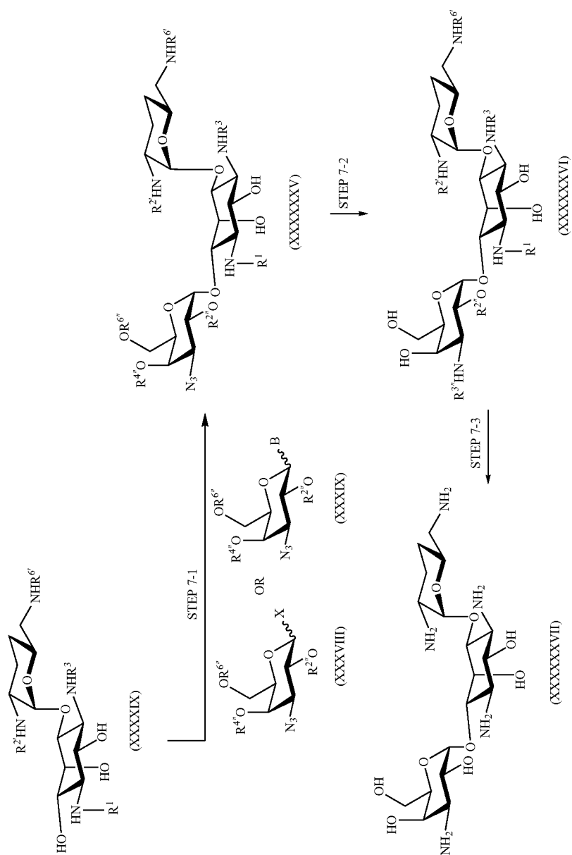
[Chemical formula 42]
