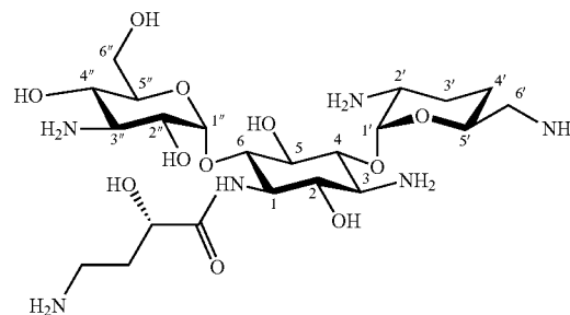
[Chemical formula 3]
