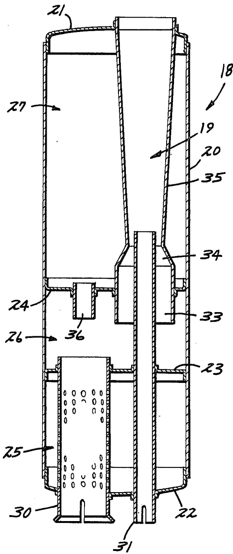
FIG. 1 PRIOR ART
